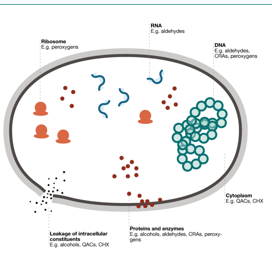
Figure 2: A simplified illustration of a bacterial cell and target sites of biocides. Abbreviations: QAC; quaternary ammonium compound, CHX; chlorhexidine dighonate, CRA; chlorine releasing agent.
