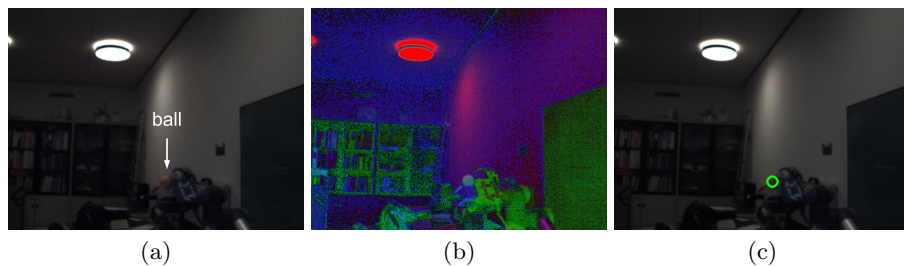
Fig. 5. Image processing for determining the 2D coordinate of a ball in the image space. (a): RGB image; (b) HSV image converted from RGB image; (c): ball detected (highlighted by green-circle) in image space.
