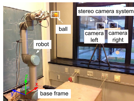
Fig. 4. Experimental setup.
