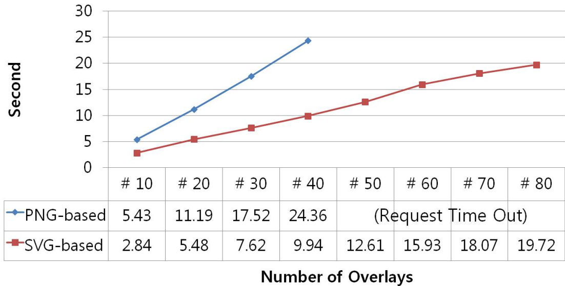
Figure 6.14: Comparison of loading time with respect to the number of overlays.
