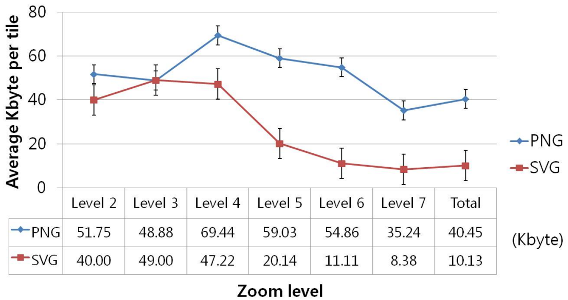
Figure 6.12: Average file size of a tile in each zoom level.
