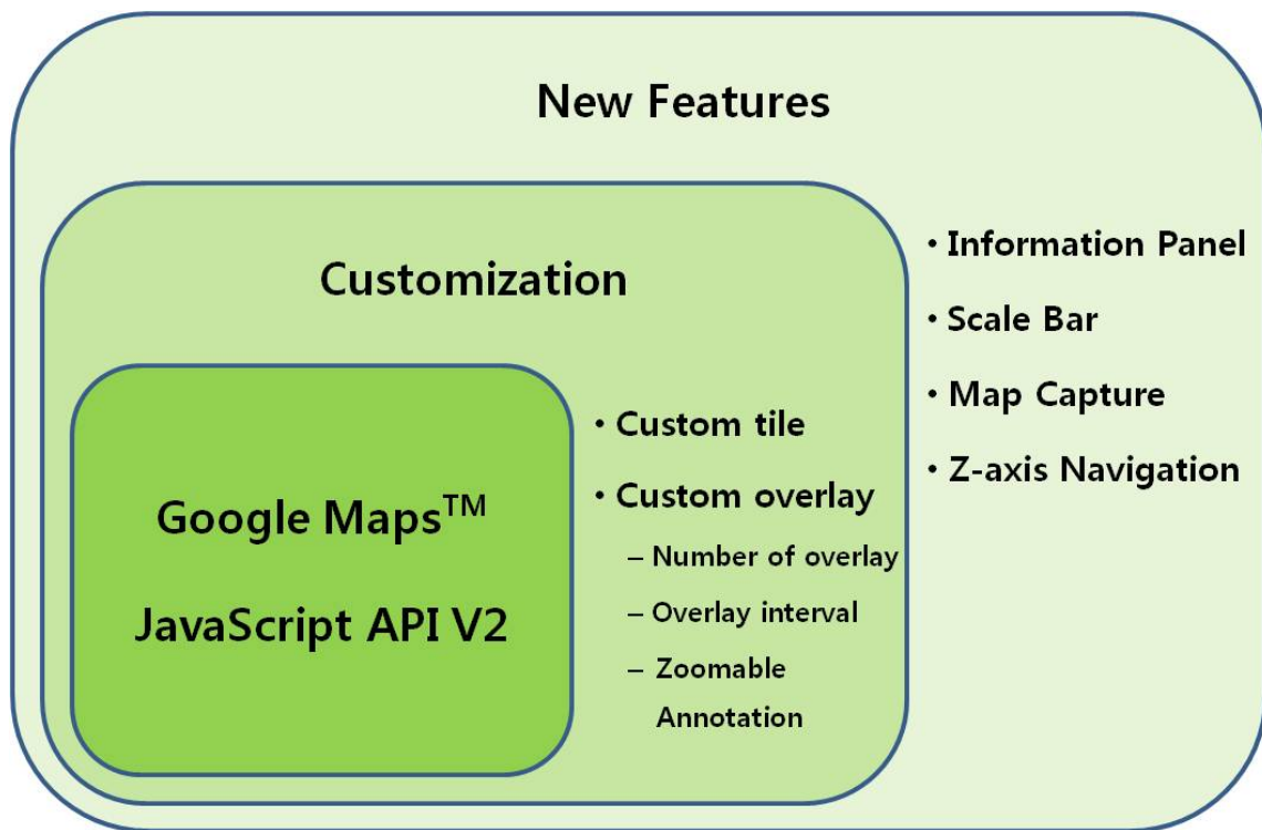
Figure 4.3: Structure of the KESMBA using Google Maps API.
