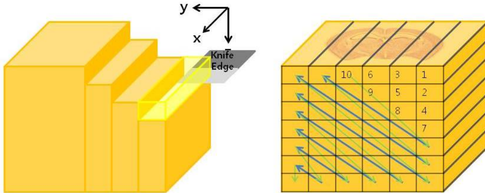
Figure 2.4: Stair-step algorithm [19]
