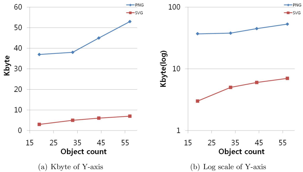
Figure 6.10: Comparison of file size of tiles with different object count and the same total object area.
