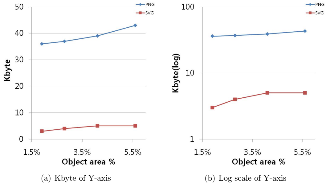
Figure 6.9: Comparison of file size of tiles with different total object area and the same object count.
