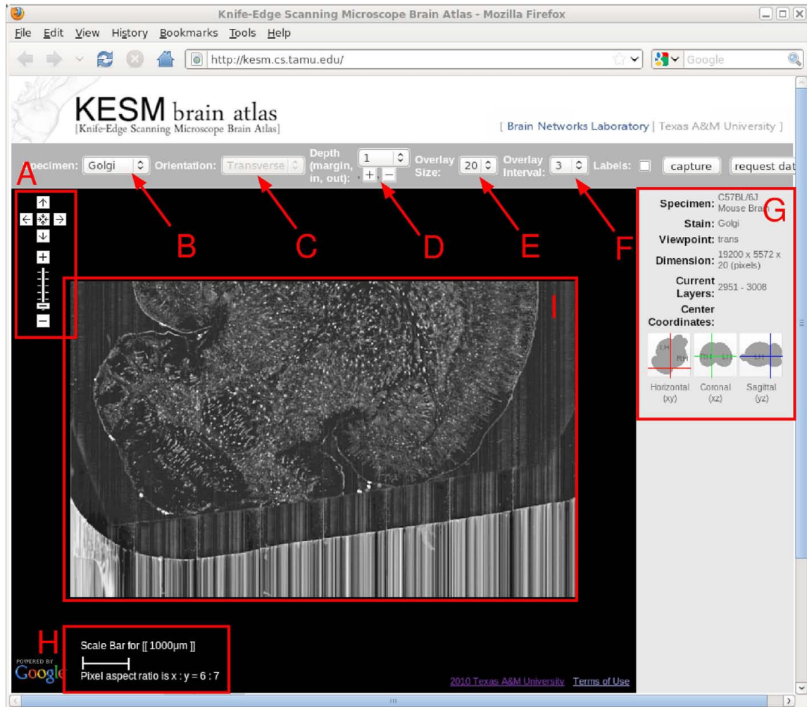
Figure 4.7: The interface of KESMBA which provides a web-based atlas service: (A) navigation control and zoom level bar, (B) and (C) data and orientation selection menu, (D) z-axis navigation control, (E) and (F) menu to select the number and interval of overlay, (G) information panel for specimen meta data and current location information, and (H) scale bar. Adapted from [9].
