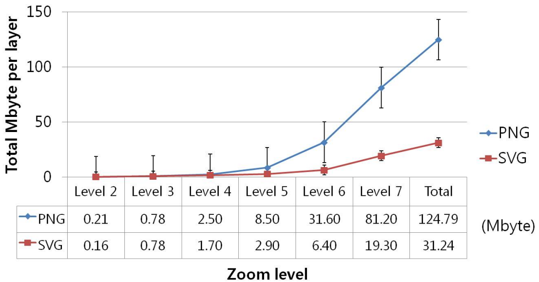
Figure 6.13: Total file size of a layer with respect to zoom level.
