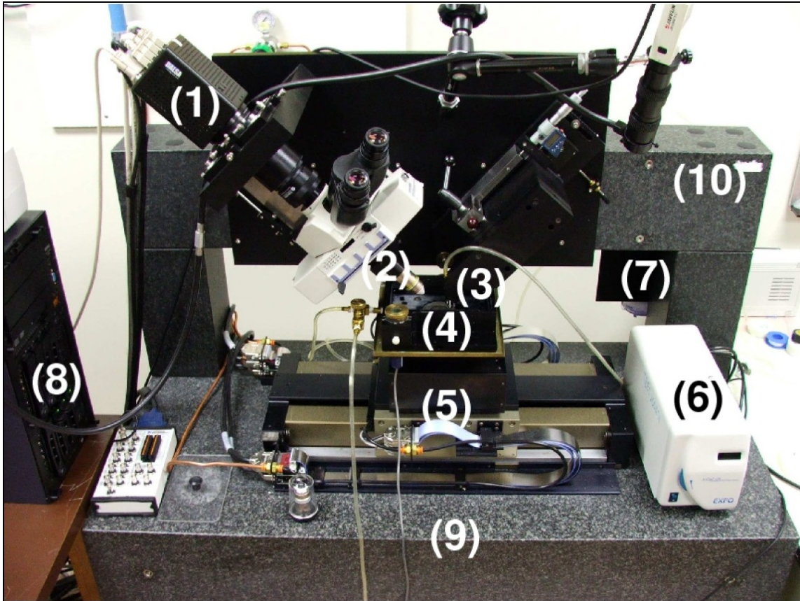
Figure 2.2: The Knife-Edge Scanning Microscope (KESM). A photo of the KESM is shown with its major components marked: (1) high-speed line-scan camera, (2) microscope objective, (3) diamond knife assembly and light collimator, (4) specimen tank (for water immersion imaging), (5) three-axes precision air-bearing stage, (6) white-light microscope illuminator, (7) water pump (in the back) for the removal of sectioned tissue, (8) PC server for stage control and image acquisition, (9) granite base, and (10) granite bridge. Adapted from [5].
