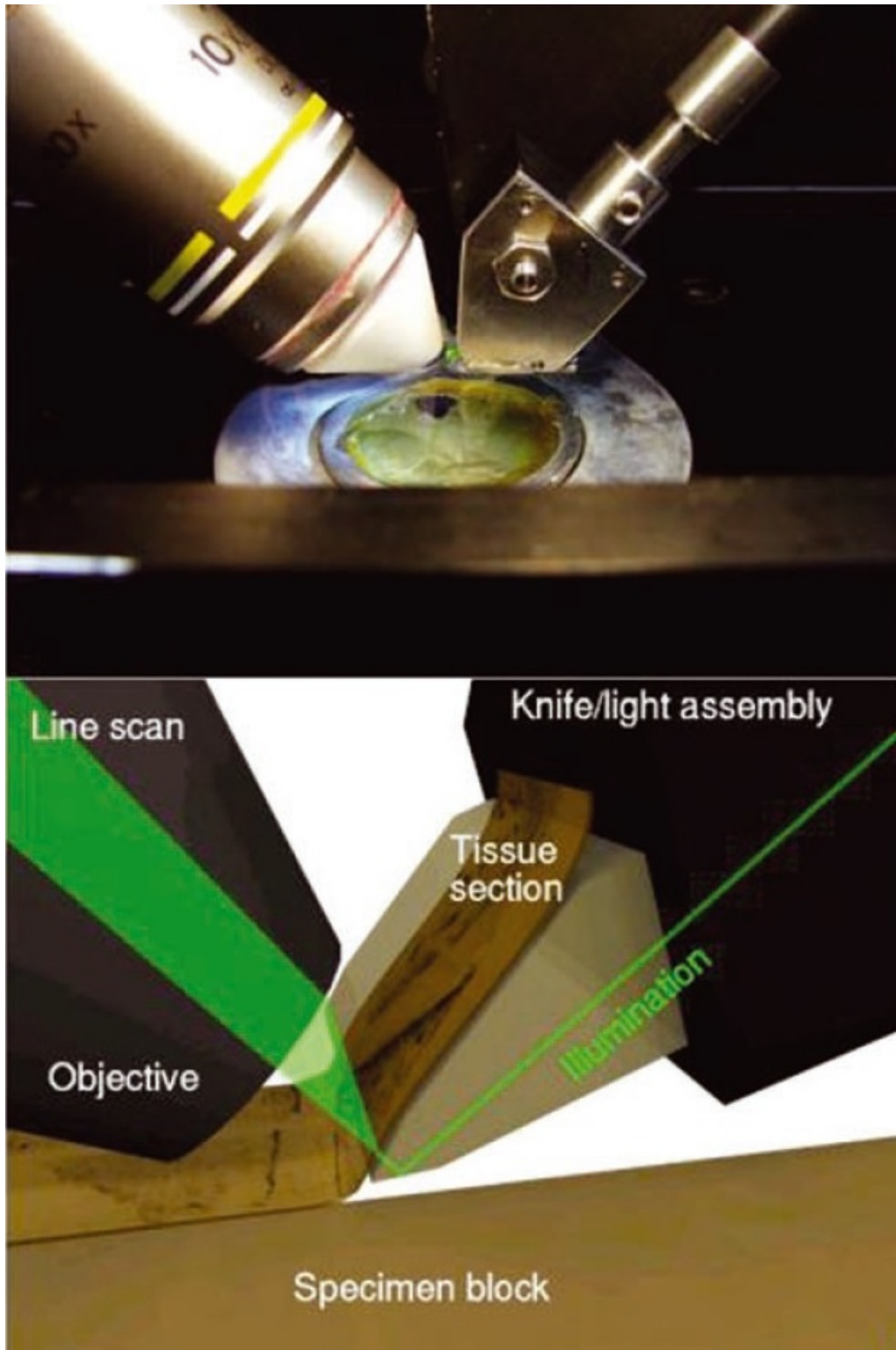
Figure 2.3: Tissue sectioning and imaging in KESM. A photograph of the objective, knife and specimen (top), and a cartoon of the illustrating light transport through the diamond knife and through the objective for imaging (bottom). Adapted from [22].
