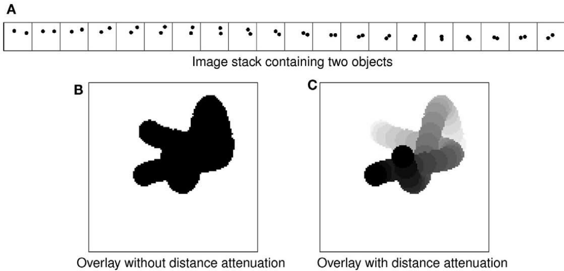
Figure 4.5: Transparent overlay with distance attenuation. (A) An image stack containing two intertwined objects are shown. (B) Simple overlay of the image stack in (A) results in loss of 3D perspective. (C) Overlay with distance attenuation helps bring out the 3D cue. Adapted from [11].
