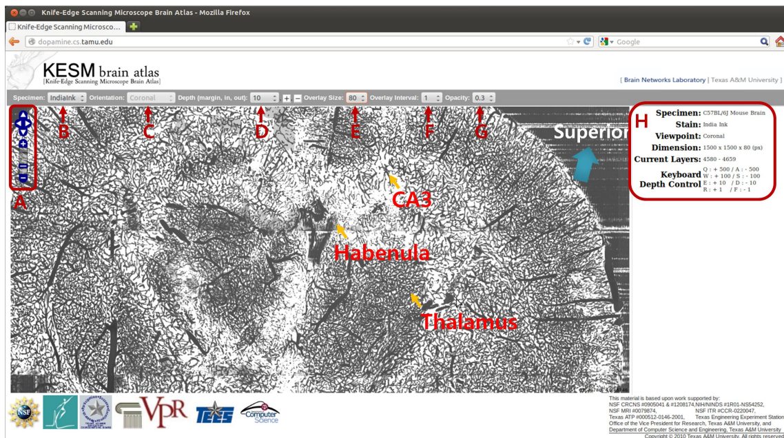
Figure 6.4: The features of the SVG-based KESMBA using OpenLayers API. (A) Navigation control and zoom level bar. (B) and (C) Data and orientation selection menu. (D) Z-axis navigation control. (E) and (F) Menu to select the number and interval of overlay. (G) Opacity option to adjust transparency level. (H) Information panel for specimen meta data and current location information.
