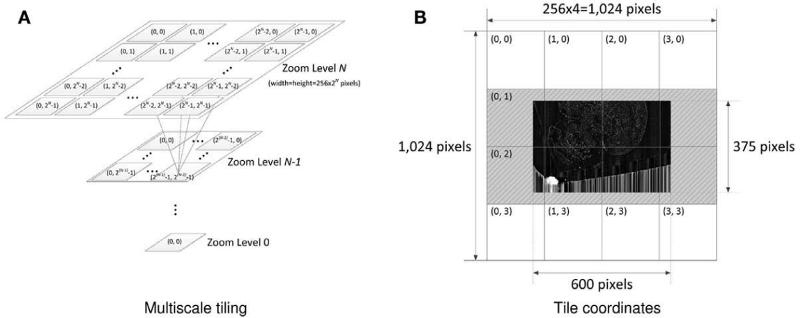
Figure 4.6: Multiscale tiling scheme. (A) Zoom level N is composed of 2^N \times 2^N tiles with each tile being 256 \times 256 pixels. (B) Example of KESM Golgi tiles in zoom level 2, where the entire brain can be displayed in a single screen. Adapted from [9].
