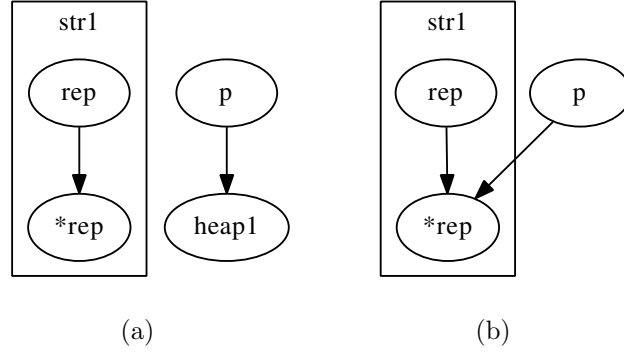
Figure 6.6. A heap object becomes part of a string, as a result of an pointer assignment \text{str1.rep} = \text{p} . Case (a) depicts the topology of the objects before the assignment and Case (b) after.
