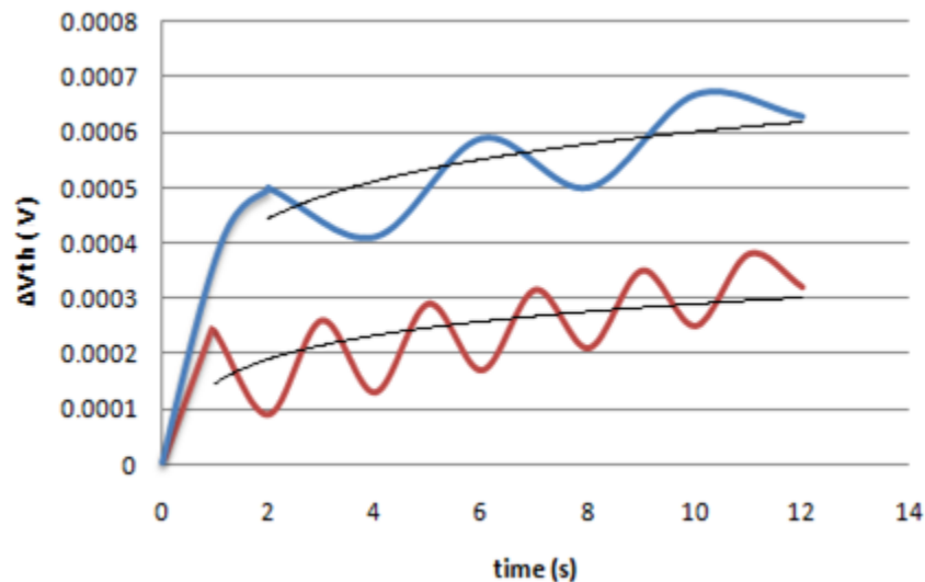
Figure 5-1 (b). RD model is frequency dependent
