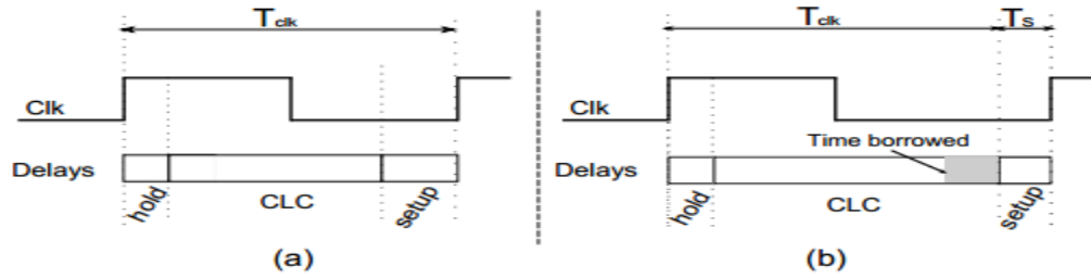
Figure 3.6 (a)Max. allowable delay of CL and FFs (b) Time borrowing by CL using setup margin of FF in the next stage [29]
