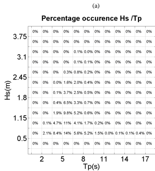
Fig. 6 Example of scatter diagram at SWMTF
