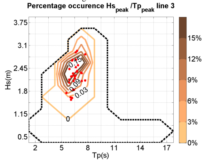
Fig. 12 Joint probability distribution of H_{s_{peak}}/T_{p_{peak}} on mooring line 3 at SWMTF (coloured solid lines), envelope of the joint probability distribution of H_s/T_p at SWMTF (black dashed line), and 30 mooring loads with the highest amplitude (red dots)
