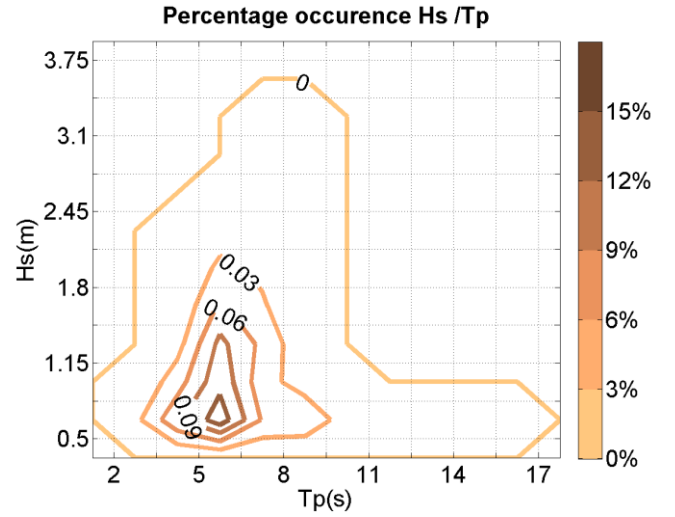
Fig. 11 Contour plot of the joint probability distribution of H_s/T_p at SWMTF
