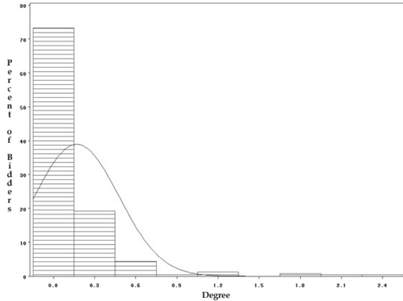
Figure 3: Degree Distribution
