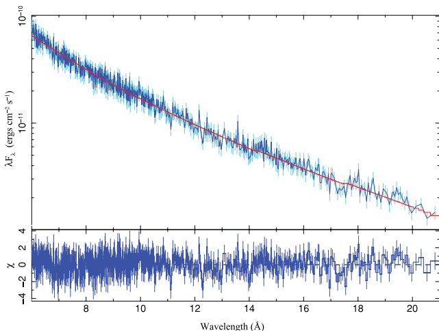
Figure 4. RGS spectrum.
