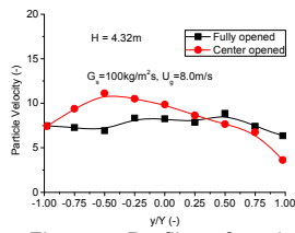
Figure 7. Profiles of particle velocity (Center opened)
