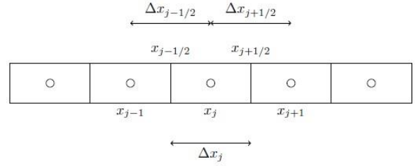
Figure 1: Control volume discretization of the 1-dimensional domain where the points x_j are chosen at the center of the block and the boundaries are located at the points x_{j\pm 1/2} .
