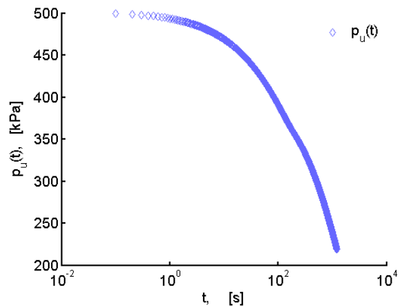
Figure 7: Pressure, p_u(t) , in the upstream reservoir is obtained from the new transport model and is plotted against time t . It shows an exponential decay of pressure with time.
