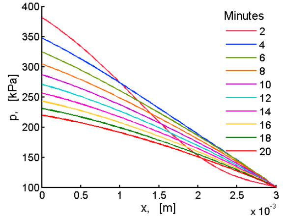
Figure 6: Numerical solutions from the new nonlinear transport model are plotted against distance x at long times (in minutes).
