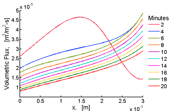
Figure 9: Plots of volumetric flux u against distance x . Here we have shown the long time behavior of u . We note that the magnitude of flux decreases with time but it decreases with the similar pattern. Moreover, the flux at the right boundary is greater than the flux at the inlet boundary.
