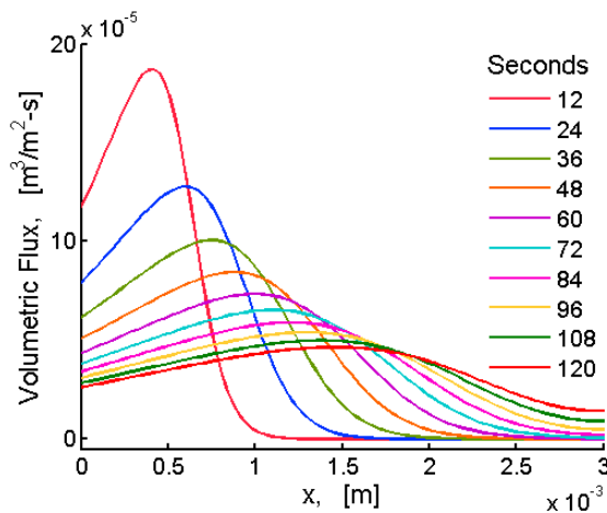
Figure 8: Volumetric flux u obtained from the new nonlinear transport model are plotted against distance x at short times (in seconds). We note that the volumetric flux greatly depends on the pressure gradient, it is very large for shorter times, say for t < 2 minutes.
