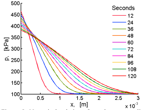
Figure 5: Numerical solutions from the new nonlinear transport model are plotted against distance x at short times (in seconds).
