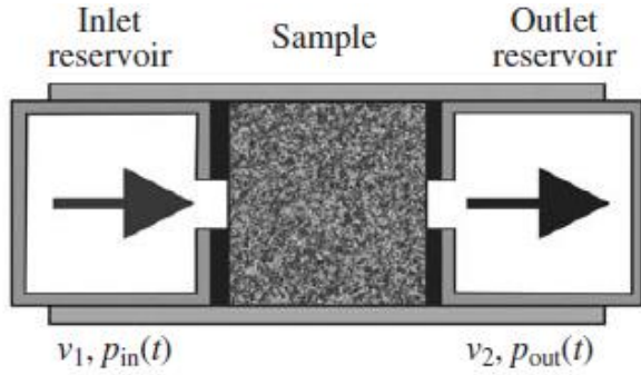
Figure 4: Transient pressure pulse test, Malkovsky [16].
