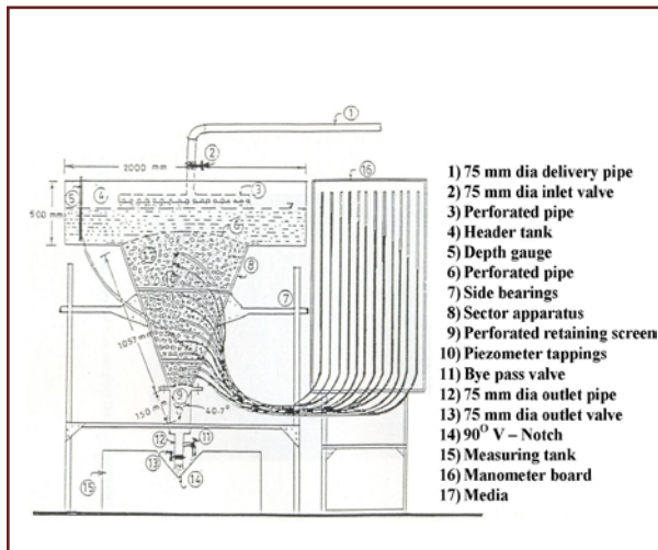
Figure 2 Converging Flow Permeameter
