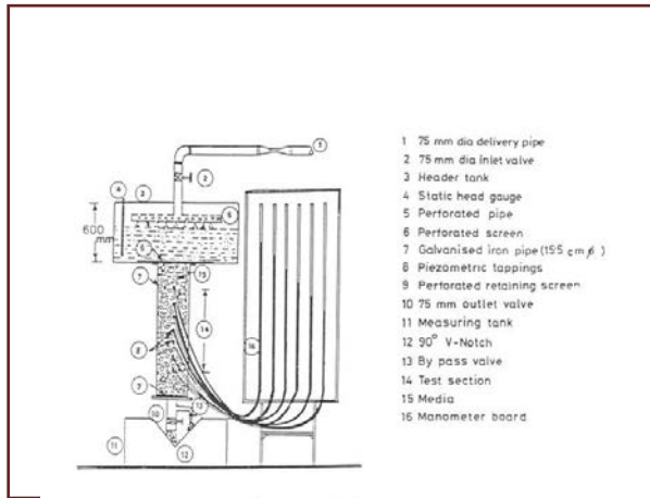
Figure 1 Parallel Flow Permeameter
