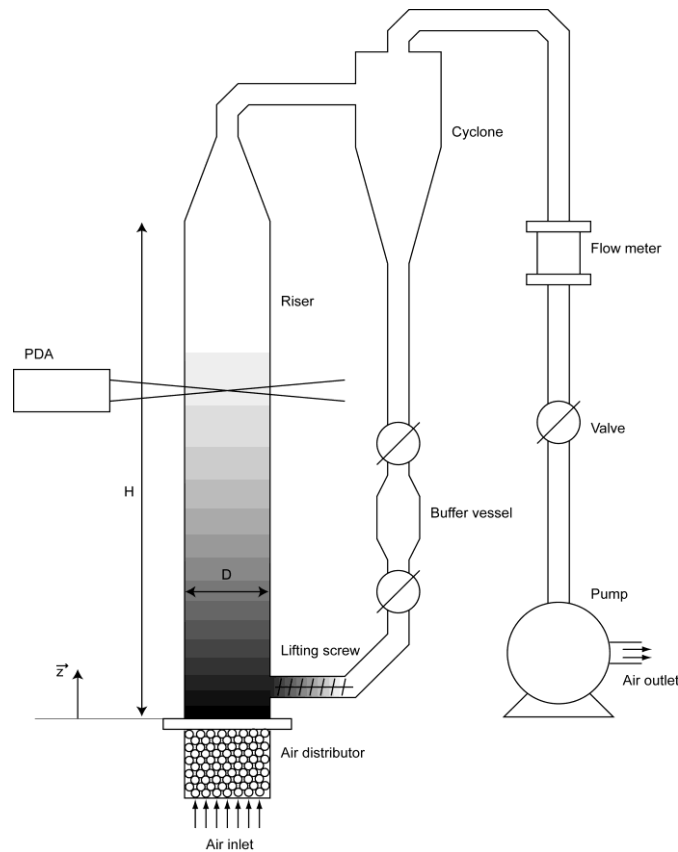
Fig.1. Schematic diagram of the circulating fluidized bed set up
