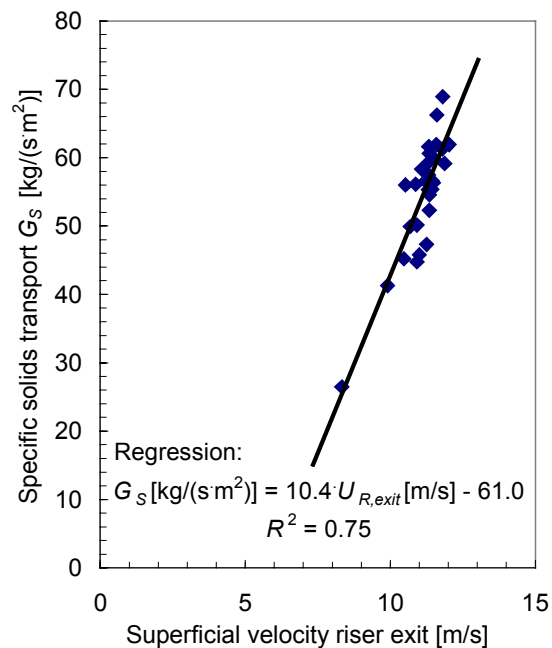
Fig. 3: Solids transport rate vs. riser exit velocity.
