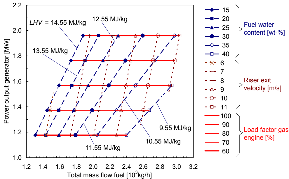
Fig. 4: CHP plant performance map 1: electric power output vs. total fuel mass flow.
