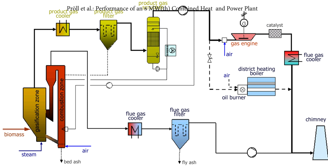
Fig. 2: The 8 MW th biomass CHP plant in Guessing/Austria.
