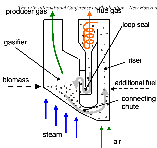
Fig. 1: Dual bed steam gasification of solid biomass.
