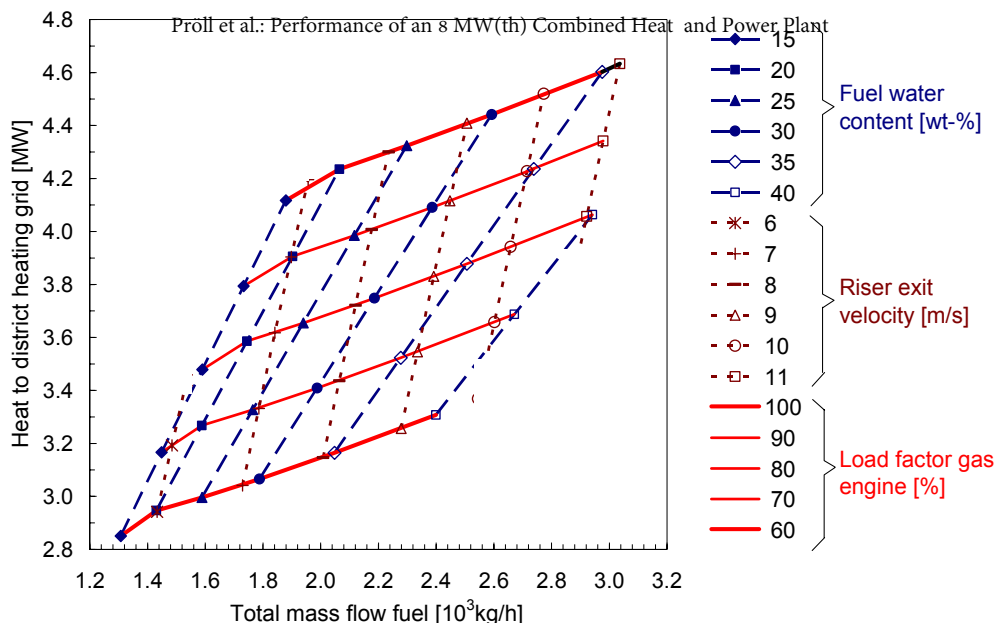
Fig. 5: CHP plant performance map 2: district heat output vs. total fuel mass flow.
