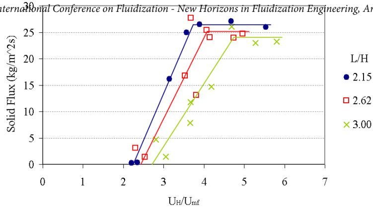
Figure 3: Changing Solid Flux with Supply Chamber Aeration and Horizontal Passage Length
