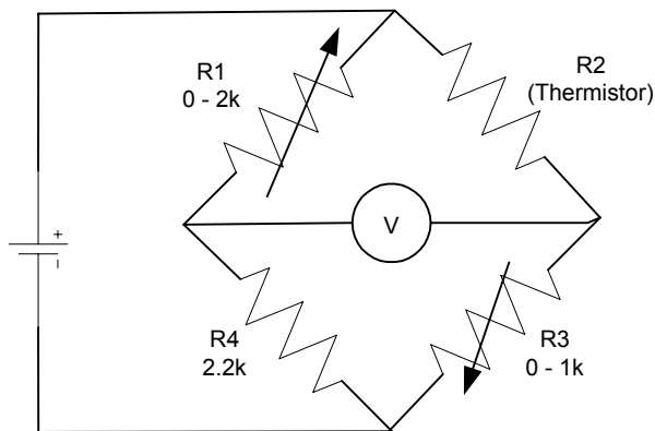
Figure 1 Thermistor bridge
