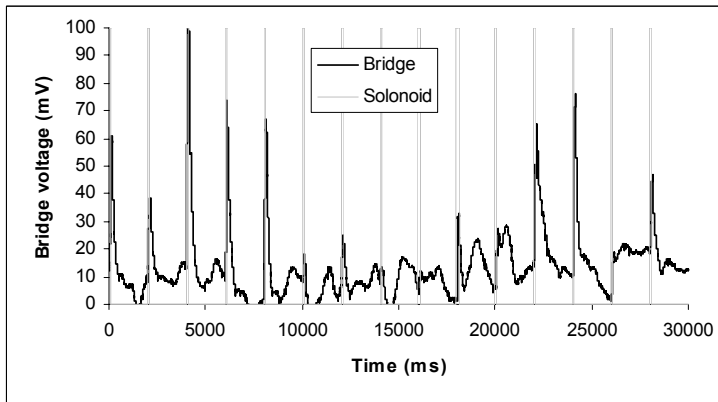
Figure 6 Typical thermistor response to helium injections
