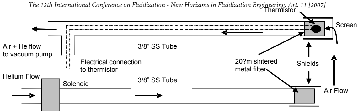
Figure 2 Thermistor and helium injection probes
