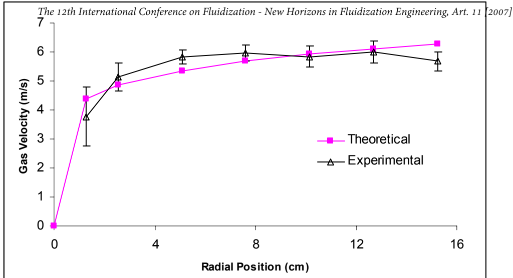
Figure 5 Probe Calibration
