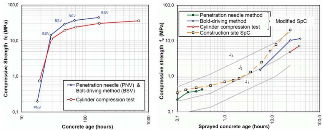
Fig. 3: Early strength development evaluated by means of penetration needle and bold-driving methods and cylinder compression tests. a) Wet mix poured in formwork, b) Sprayed concrete on the tunnel sidewall
