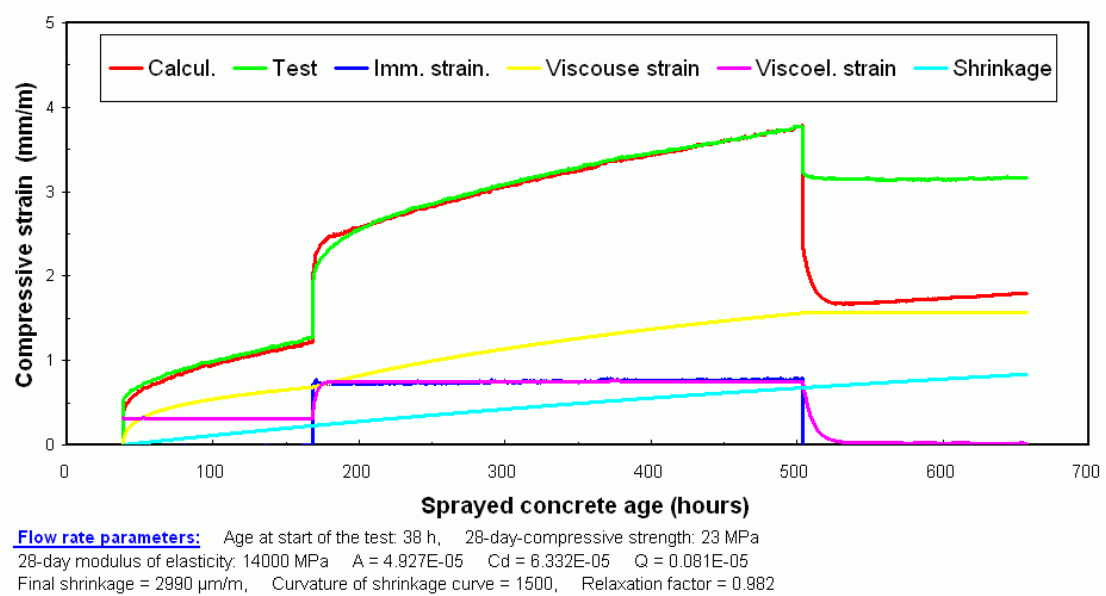
Fig. 8: Flow rate parameter identification for the average value curve for longitudinal compressive strain
