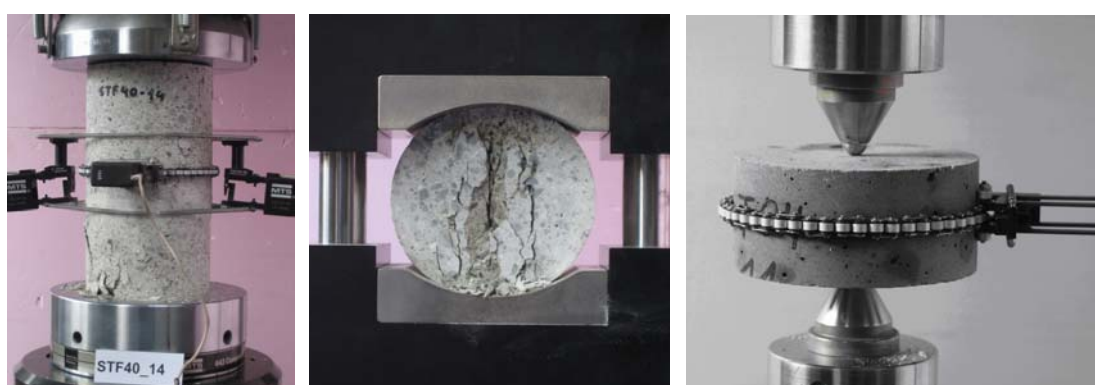
Fig. 17: a) Uniaxial compression test, b) Brazilian test, c) Point load test
