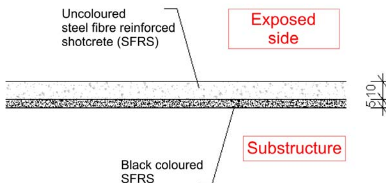
Fig. 15: Wear monitoring with differently coloured layers of sprayed concrete
