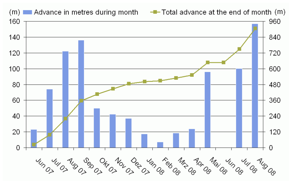
Fig. 11: Advance rates at Stetten
