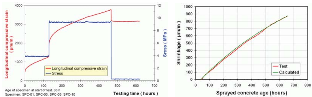
Fig. 7: Average value curves of the a) longitudinal compressive strain and stress and b) shrinkage strain
