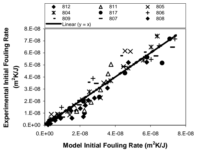
Figure 9: Comparing Experimental and Modified Model Initial Fouling Rate Results
