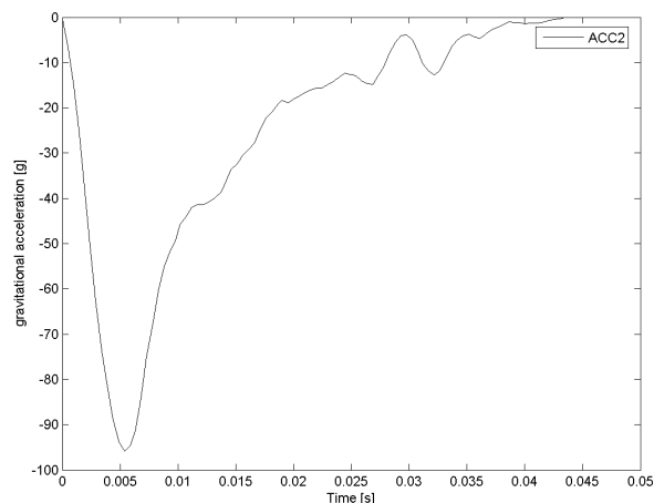
Figure 6: Typical deceleration history of low-energy rockfall impact.
