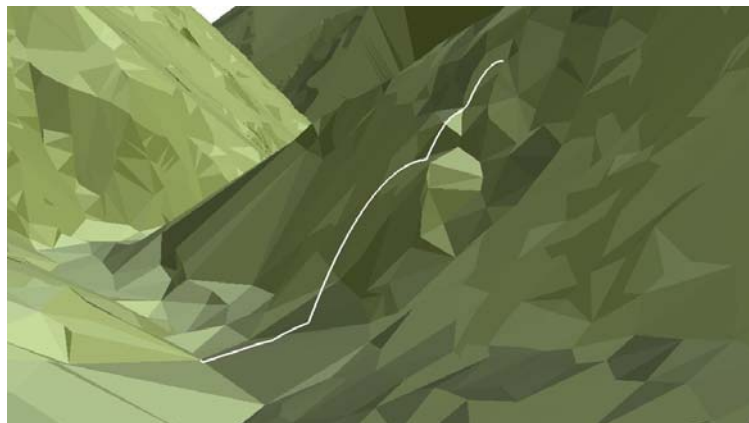
Figure.3 3D representation of rock fall analysis in a GIS environment, (Charalambous 2006).
