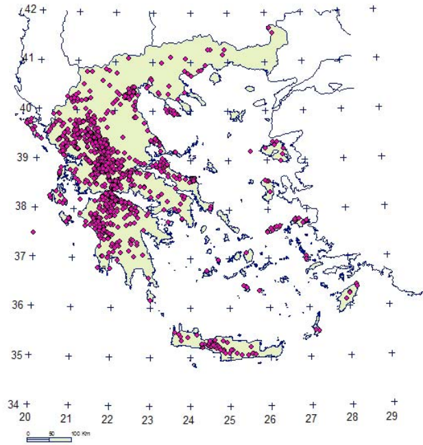
Figure.1 Landslide distribution in Greece.
