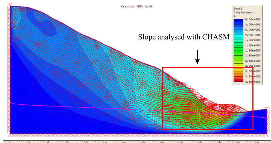
Figure.4 Displacement analysis using PHASE2.
