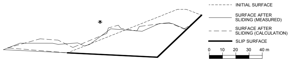
Figure 6. Initial configuration, computed final configuration with the 2-slide analysis and measured final configuration.
