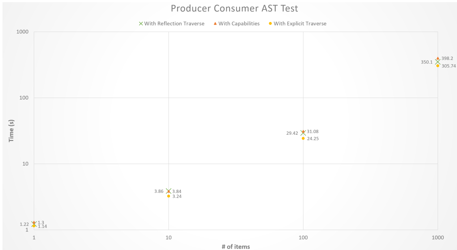
Figure 6.4: Producer-Consumer Capability/Traverse Benchmark
