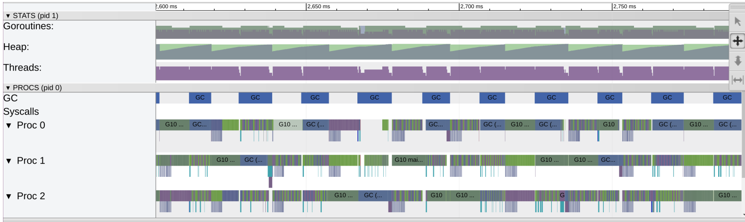
Figure 6.1: Base Goroutine Trace (NBody)
