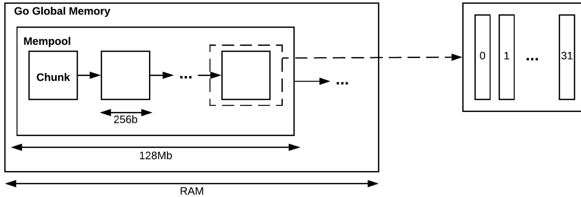
Figure 3.3: GoA Memory Layout
