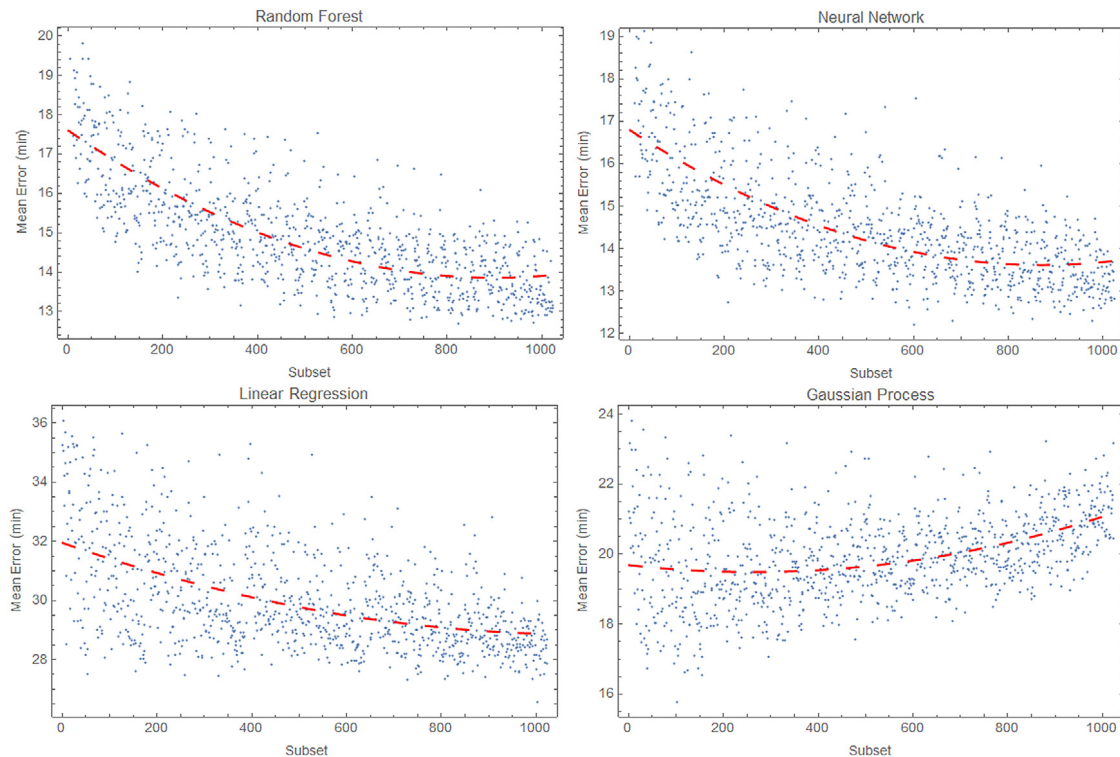
Fig. 8. Mean error of each subset of features and each algorithm: evolution of the average error of the predictors trained as the number of features considered increases.
