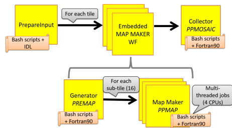
(a) PPMAP Workflow implemented as a parameter sweep workflow embedding a parameter sweep map maker workflow.
