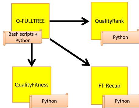
Figure 5: Q-FULLTREE Workflow schema.
