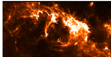
(b) PPMAP sample output of differential column density on tiles at longitude from 136 to 138 degrees.
