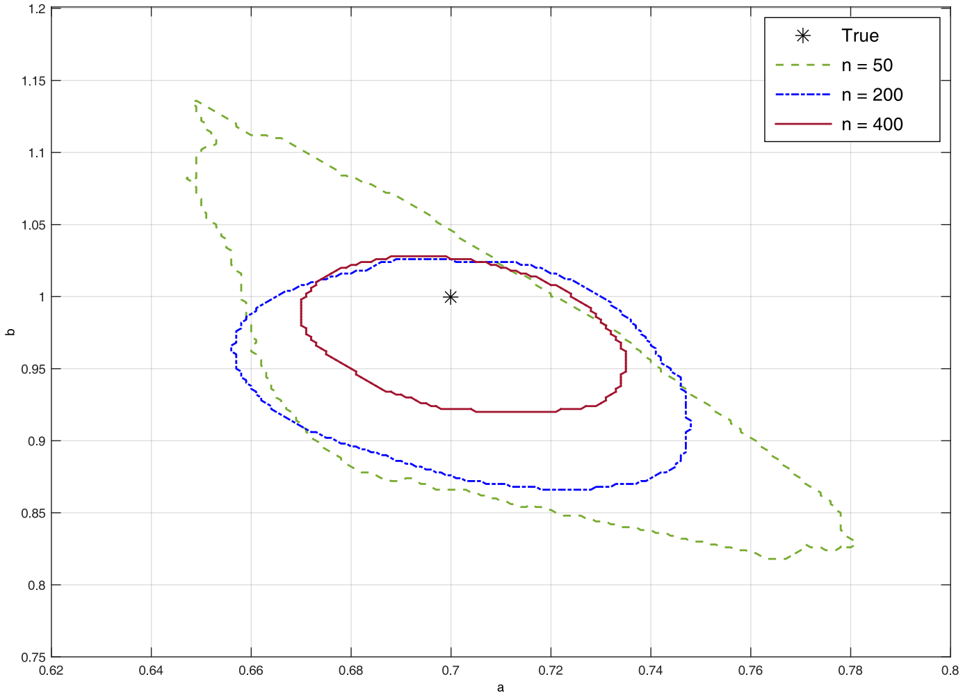
Fig. 1. 95% confidence regions built by SPCR with k=2 and l=2 .
