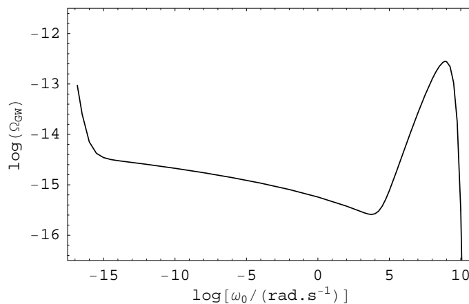
Figure 1. Gravitational-wave spectrum for \lambda_\phi = 10^{-13} , M = 3.16 \times 10^{-14} m_p ; g = 6.3 \times 10^{-4} , m = 0.01 m_p , \lambda_\chi = 1 and \mu = 0.1 .
