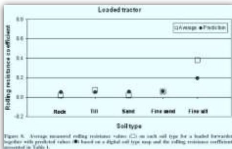
Figure 8. Average measured rolling resistance values (□) on each soil type for a loaded tractor, together with predicted values (●) based on a digital soil type map and the rolling resistance coefficient presented in Table 1.
