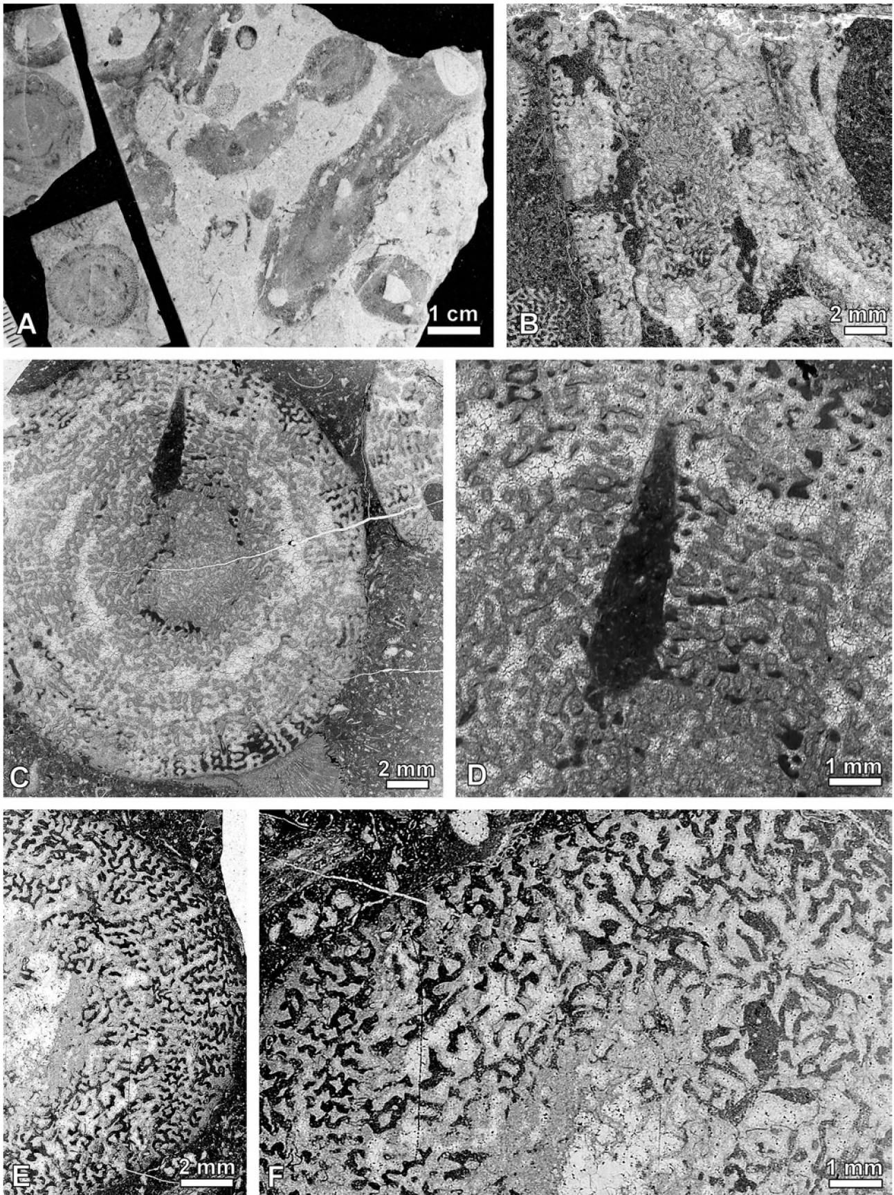
Fig. 9. A–D – Eocomoseris rauenii Löser, No. 4758/7: A – polished section of several colony branches; B – fragment of branch in longitudinal section (thin section No. 4758/7b); C – thin section across the branch (No. 4758/7a) showing microsolenid skeleton structure; D – enlarged view of fragments from Fig. 9C. E, F – Eocomoseris rauenii Löser, No. 4760/9: E – fragment of branch in transverse section; F – branch in transverse section (4760/9a) showing small subthamnasterioid corallites
