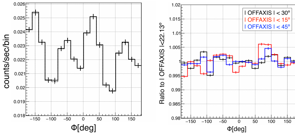
Fig. 12. Azimuth angle distributions of simulation data. Left: The azimuth angle distributions of the simulation data with the \text{OFFAXIS} selection of -22.13 < \text{OFFAXIS} < +22.13 and -30^\circ < \text{OFFAXIS} < +30^\circ are shown in the solid line and the dotted line, respectively. The normalization for the -30^\circ < \text{OFFAXIS} < +30^\circ selection is scaled. Right: The dependence of the azimuth angle distribution on the selected \text{OFFAXIS} value. This is shown as the ratio to the \text{OFFAXIS} selection of three values to that limited to -22.13 < \text{OFFAXIS} < +22.13 . The black, red, and blue points show the results for \text{OFFAXIS} selections of -30^\circ < \text{OFFAXIS} < +30^\circ , -15^\circ < \text{OFFAXIS} < +15^\circ , and -45^\circ < \text{OFFAXIS} < +45^\circ , respectively.
