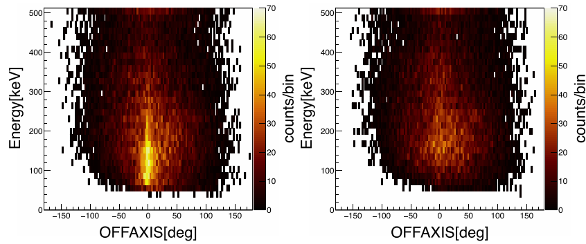
Fig. 4. Two-dimensional histograms of Compton-reconstructed events. The relation between OFFAXIS and energy is shown. The left-hand panel is the histogram made from the events during the Crab GTI; the right-hand panel is prepared from the events collected one day earlier than the Crab GTI.
