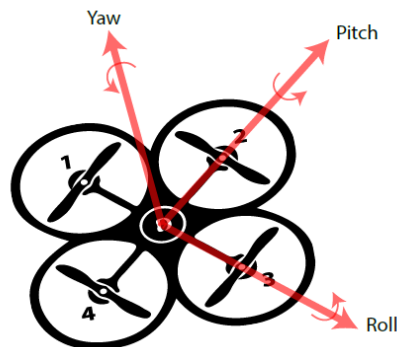
Figure 2. Euler angles for quadrotor
