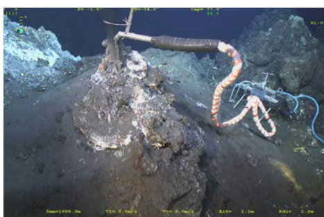
Figure 3 : BARS monitors the temperature and chlorinity of the hot hydrothermal fluid
