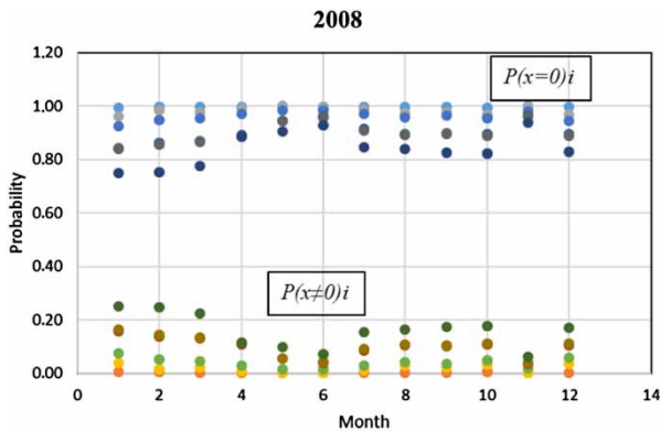
Figure 6 | Probability that IPR may have occurred on a monthly basis, downstream of the flow measurement sections in the Llobregat River during 2008.
