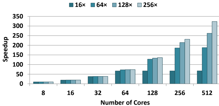
Figure 6.5 Canneal performance as we modify r ; x-axis shows the number of cores.
