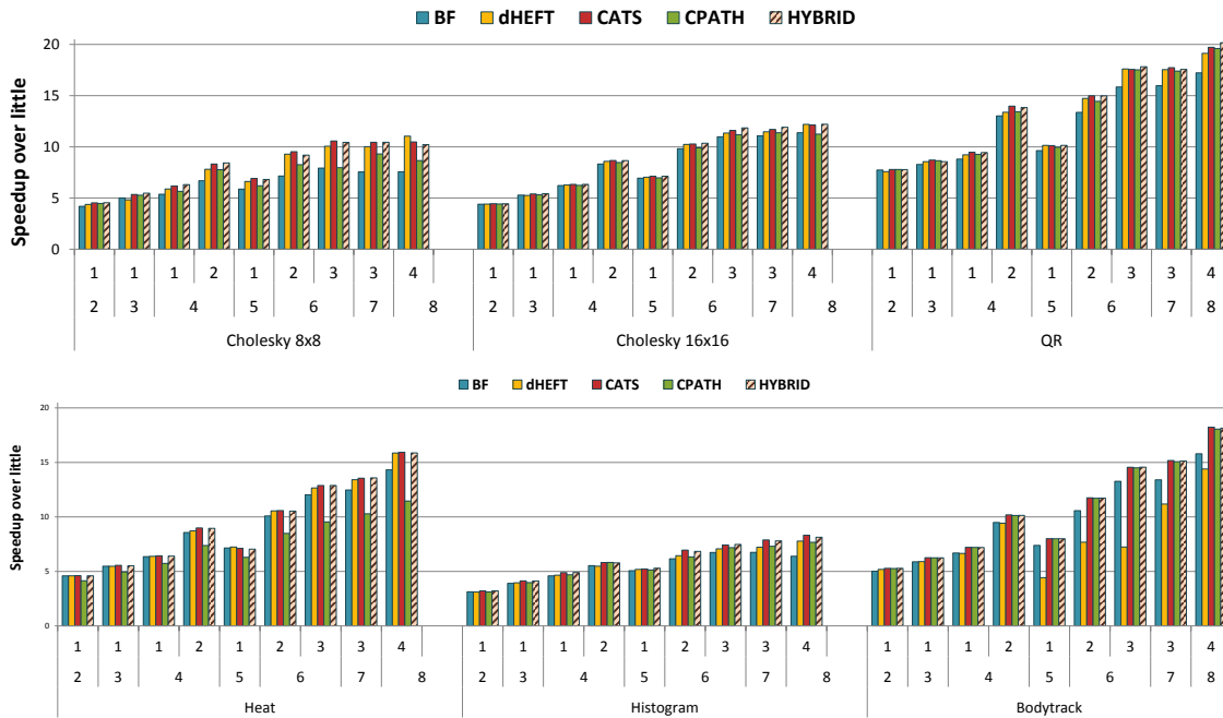
Figure 5.10 Speedups obtained for each scheduler and each application
