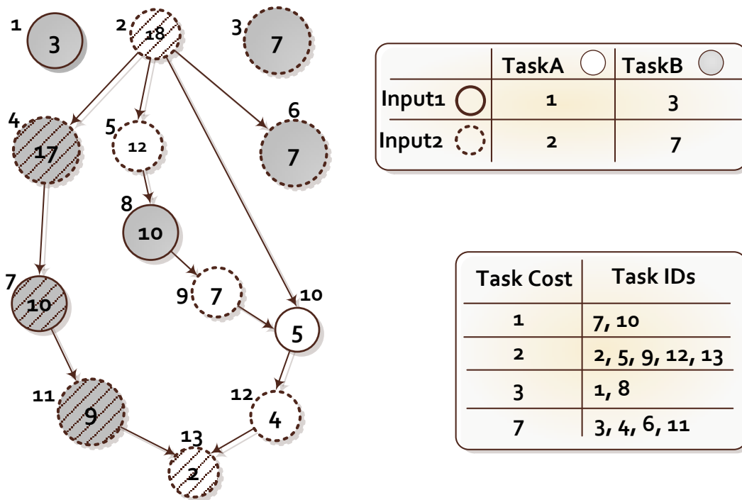
Figure 5.3 Priority assignment with CPATH taking into account the task costs. Task costs are assumed known and are shown in the tables.
