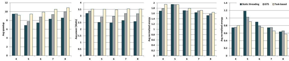
Figure 4.5 Average results when running on 4 to 8 cores with 4 of them big. Speedup is over 1 little core. Static threading on 4 little cores is the baseline of energy consumption and EDP
