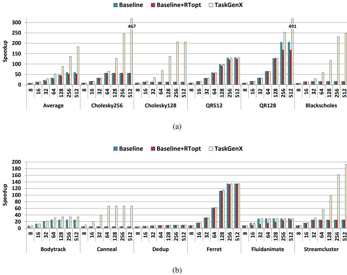
Figure 6.4 Speedup of TaskGenX compared to the speedup of Baseline and Baseline+RTopt for each application for systems with 8 up to 512 cores. The average results of (a) show the average among all workloads shown on (a) and (b)
