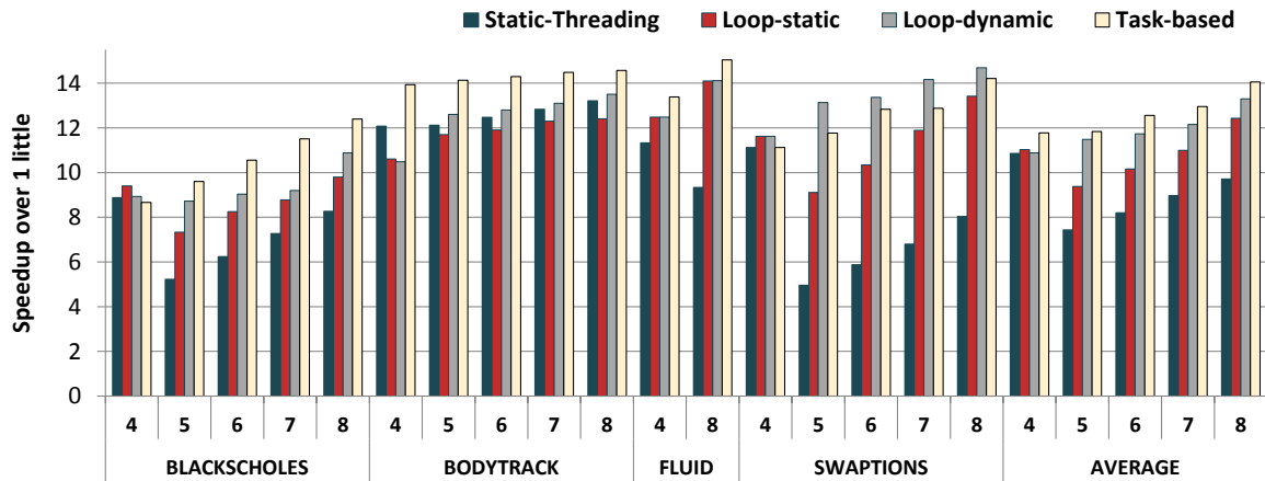
Figure 4.8 Speedup over 1 little core when running on 4 to 8 cores and 4 of them are big. Four different programming models are considered: Static threading using pthreads, parallel loops with static scheduling (loop static), parallel loops with dynamic scheduling (loop dynamic), and a task-based solution with dynamic scheduling (task-based).
