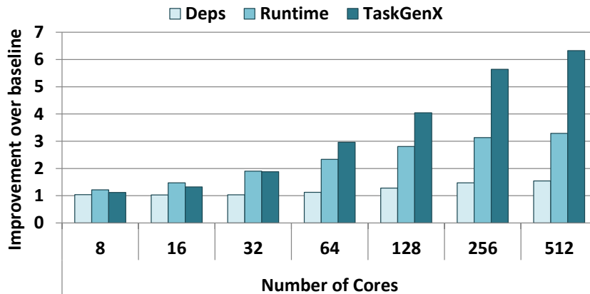
Figure 6.7 Average improvement of hardware-software proposals over Nanos++ runtime running on each number of cores; x-axis shows the number of cores.
