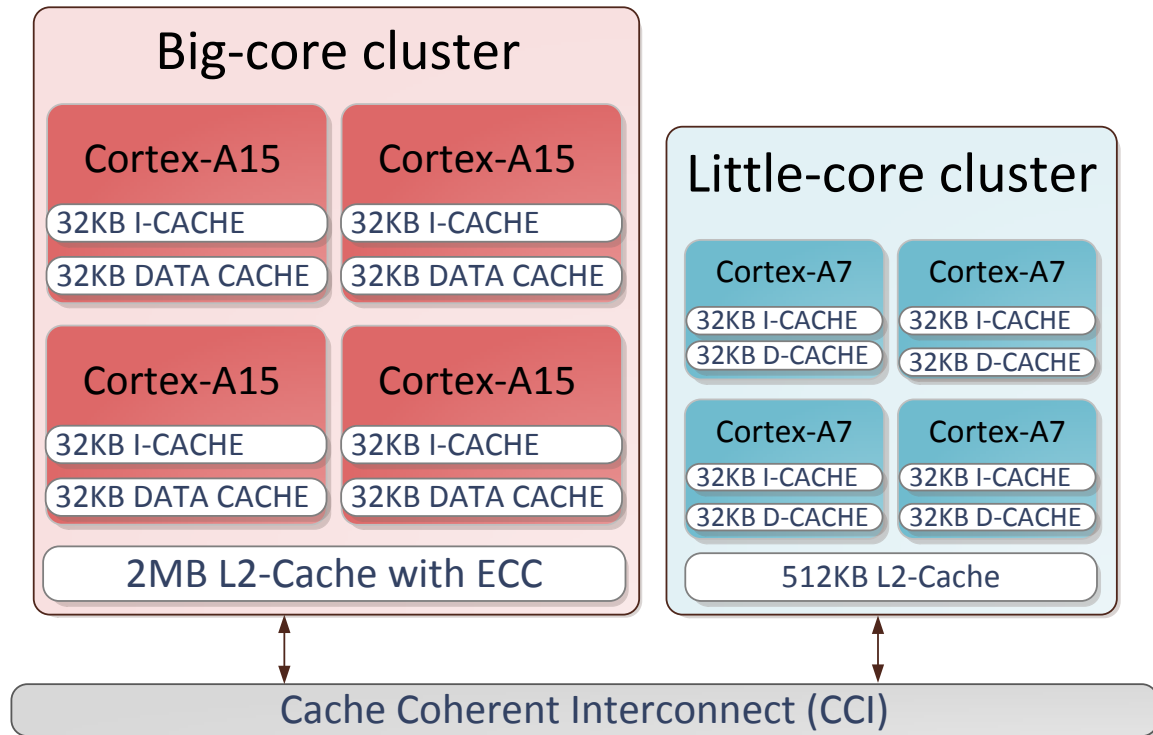
Figure 3.1 Samsung Exynos 5422 processor with Arm big.LITTLE architecture.
