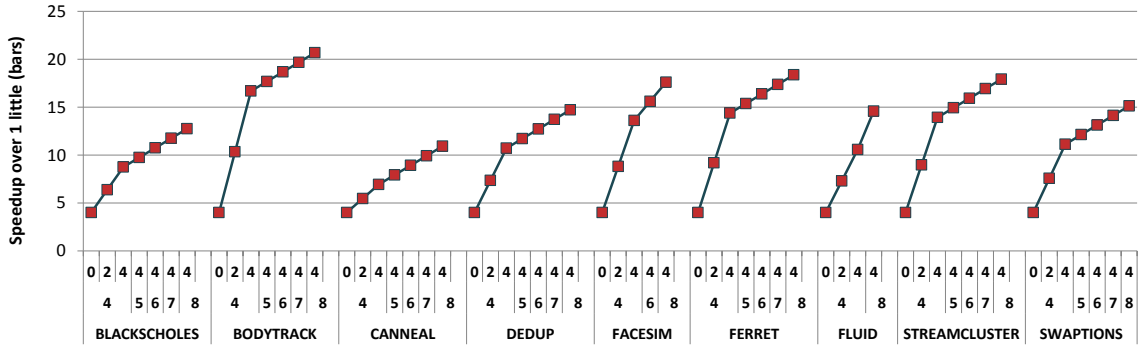
Figure 4.1 Ideal speedup over 1 little core according to Equation 4.7. Numbers at the bottom of x axis show the total number of cores, numbers above it show the number of big cores
