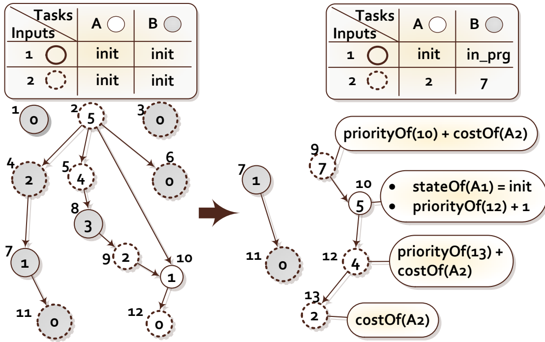
Figure 5.4 Priority assignment with HYBRID scheduler. Priority update when the edge between tasks 12 and 13 is created
