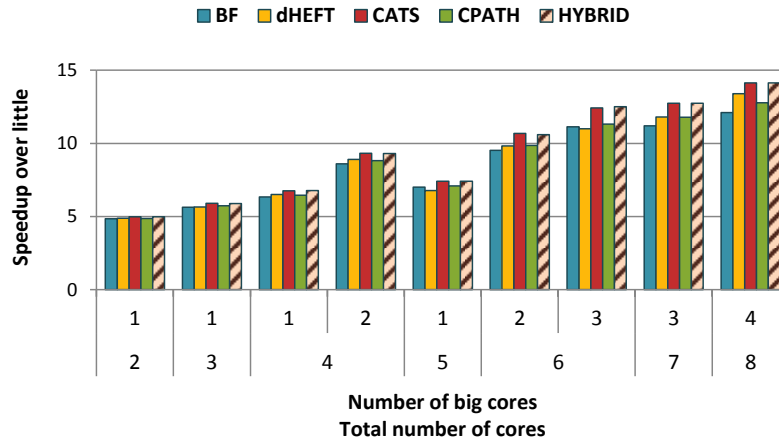
Figure 5.9 Average speedups obtained for each scheduler
