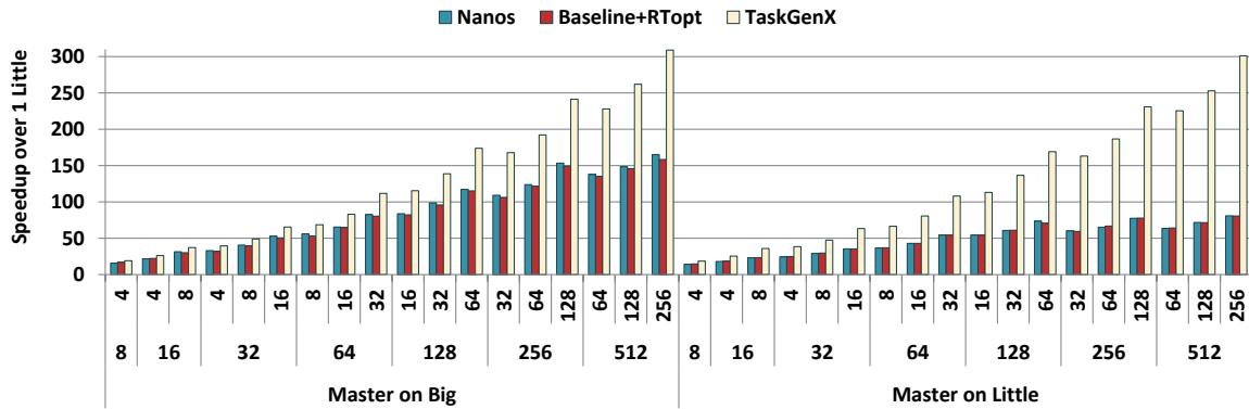
Figure 6.6 Average speedup among all 11 workloads on heterogeneous simulated systems. The numbers at the bottom of x axis show the total number of cores and the numbers above them show the number of big cores. Results are separated depending on the type of core that executes the master thread: a big or little core.
