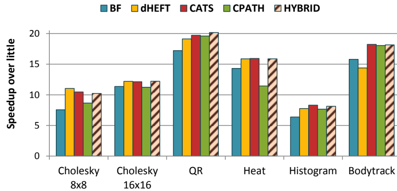
Figure 5.8 Speedup of CATS, CPATH, HYBRID, dHEFT and BF on 8 cores.
