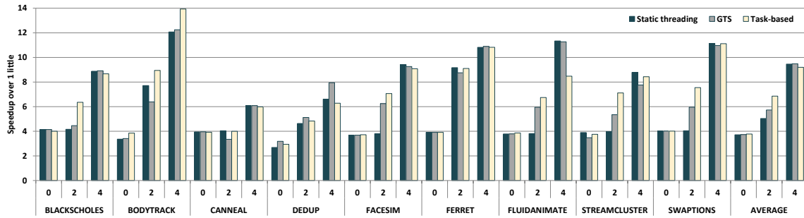
Figure 4.2 Execution time speedup over 1 little core for systems that consist of 4 cores in total with 0, 2 and 4 big cores. Different schedulers at the application ( static threading ), OS ( GTS ) and runtime ( task-based ) levels are considered.
