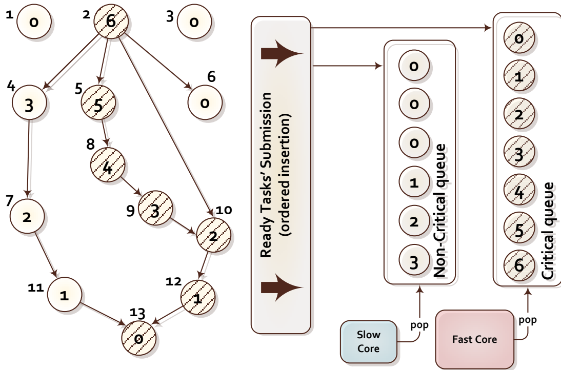
Figure 5.1 CATS overview. Nodes are marked with the bottom level of each task. Pattern-filled nodes mark the critical tasks.
