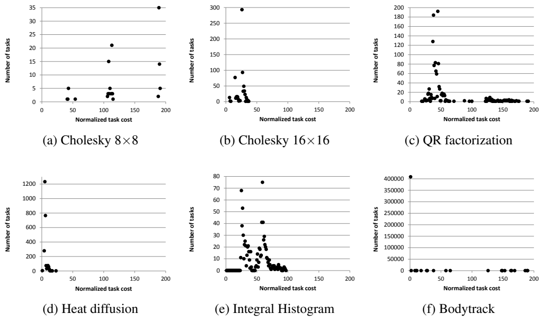
Figure 5.6 Task cost distribution for each application. Results are based on 4BIG-core executions. X axis shows the cost of the tasks and y axis shows the number of tasks with the corresponding task cost.
