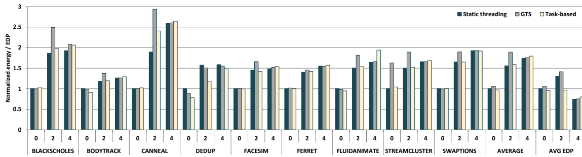
Figure 4.4 Normalized energy consumption and average EDP on a 4-core system with 0, 2, and 4 big cores. Static threading on 4 little cores is the baseline in both cases.
