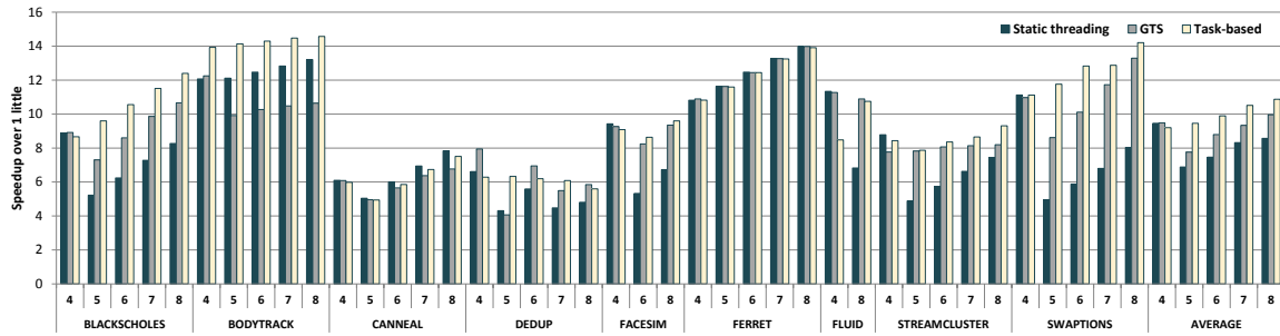
Figure 4.6 Speedup over 1 little core when running on 4 to 8 cores and 4 of them are big
