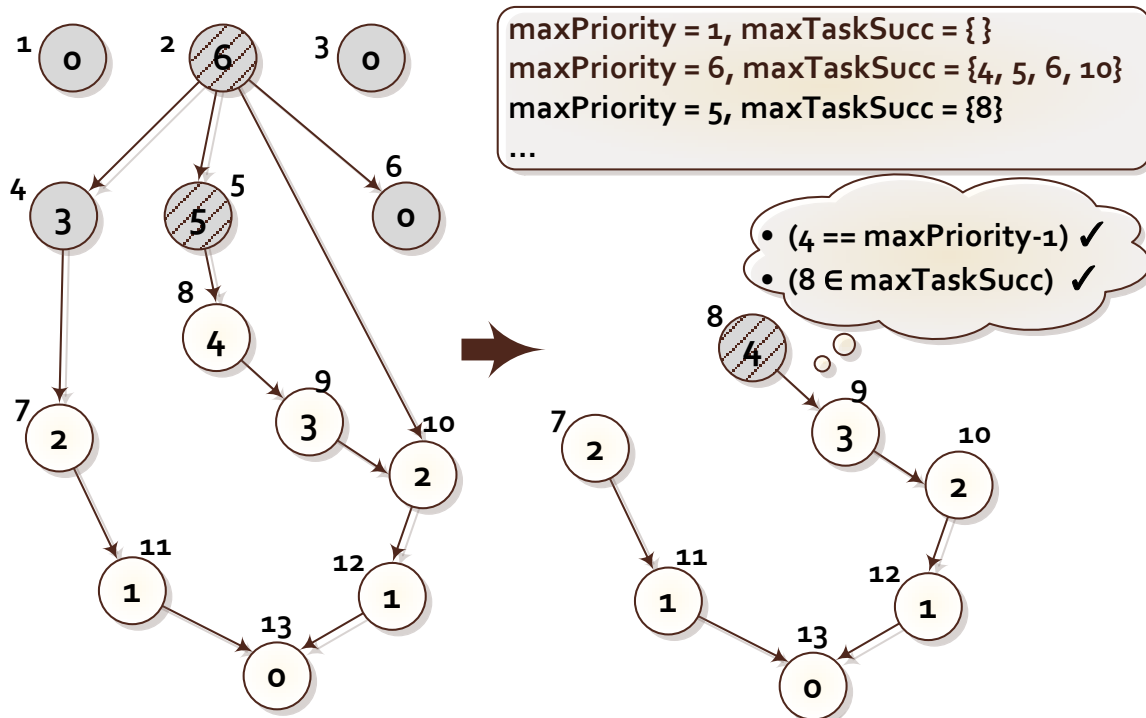
Figure 5.2 Task submission with CATS. Gray nodes indicate finished tasks and pattern-filled nodes indicate critical tasks.
