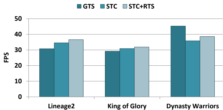
Figure 7.1 Median frames per second (FPS) results for each game (x axis) and scheduling set-up (series).
