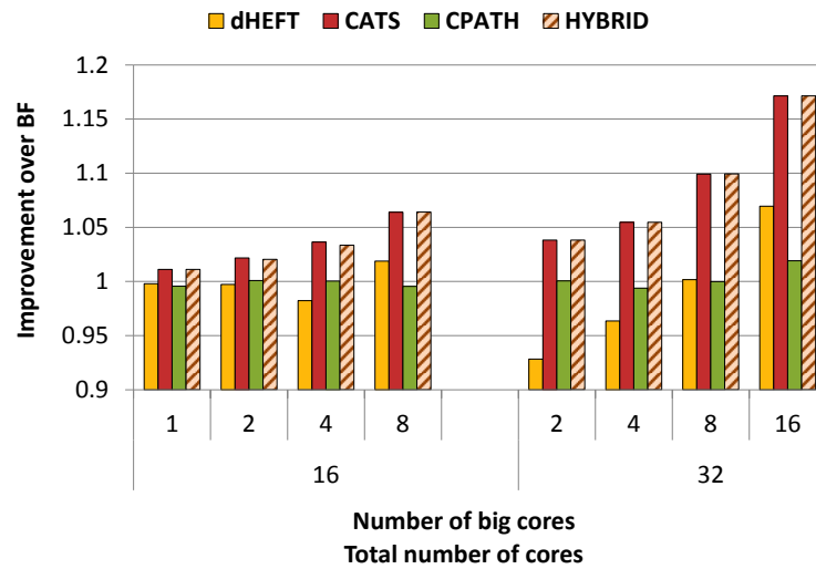
Figure 5.11 Improvement of heterogeneous schedulers over BF for simulated 16 and 32 core heterogeneous systems for Cholesky 32 \times 32 .
