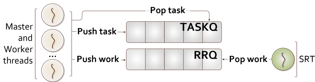
Figure 6.2 Communication mechanism between master/workers and SRT threads.
