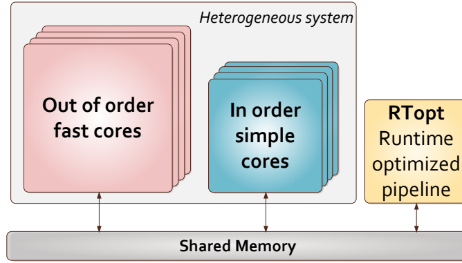
Figure 6.3 SoC architecture including three types of cores: out of order, in-order and RTopt.
