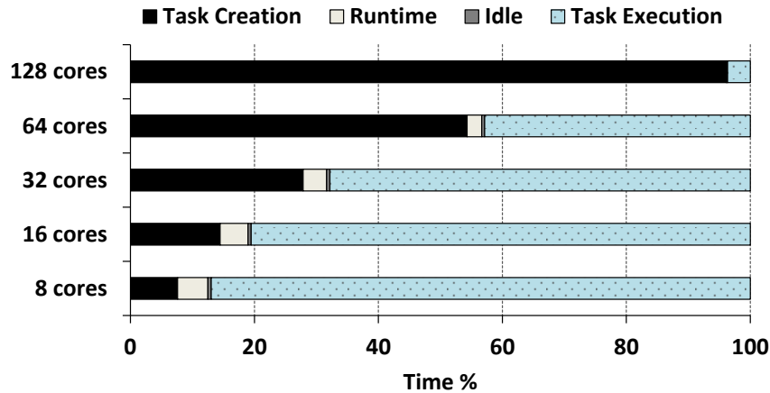
Figure 6.1 Master thread activity for Cholesky as we increase the number of cores.
