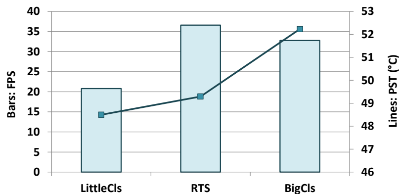
Figure 7.4 Comparison of the FPS-PST trade-offs for different scheduling policies running on top of STC.
