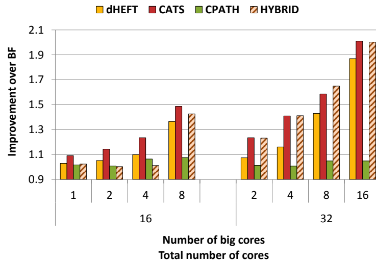
Figure 5.13 Improvement of heterogeneous schedulers over BF for simulated 16 and 32 core heterogeneous systems for heat diffusion.
