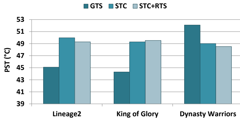
Figure 7.2 Prescribed surface temperature (PST) results for each game (x axis) and scheduling set-up (series).
