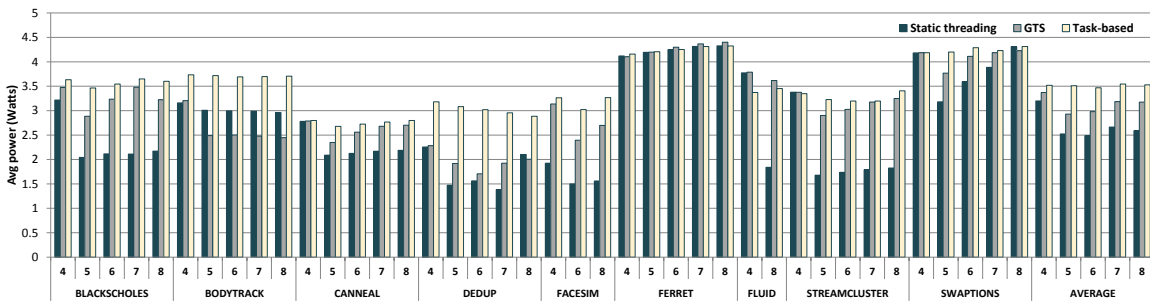
Figure 4.7 Average power when running on 4 to 8 cores and 4 of them are big
