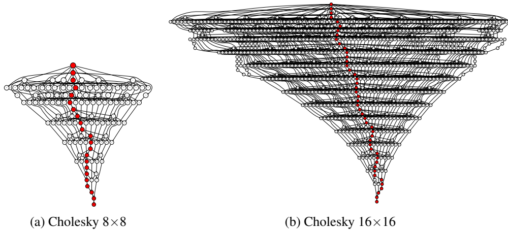
Figure 5.5 Cholesky factorization task dependency graphs.
