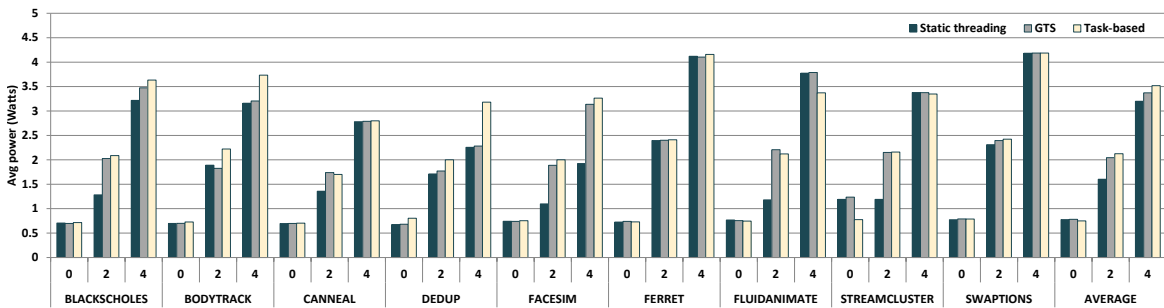
Figure 4.3 Average power measurements on a 4-core system with 0, 2, and 4 big cores.
