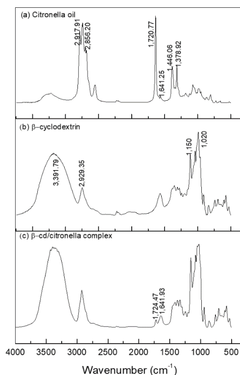
Figure 4. Spectroscopy in the infrared region of: (a) citronella oil, (b) \beta CD, (c) \beta CD–citronella oil complex.
