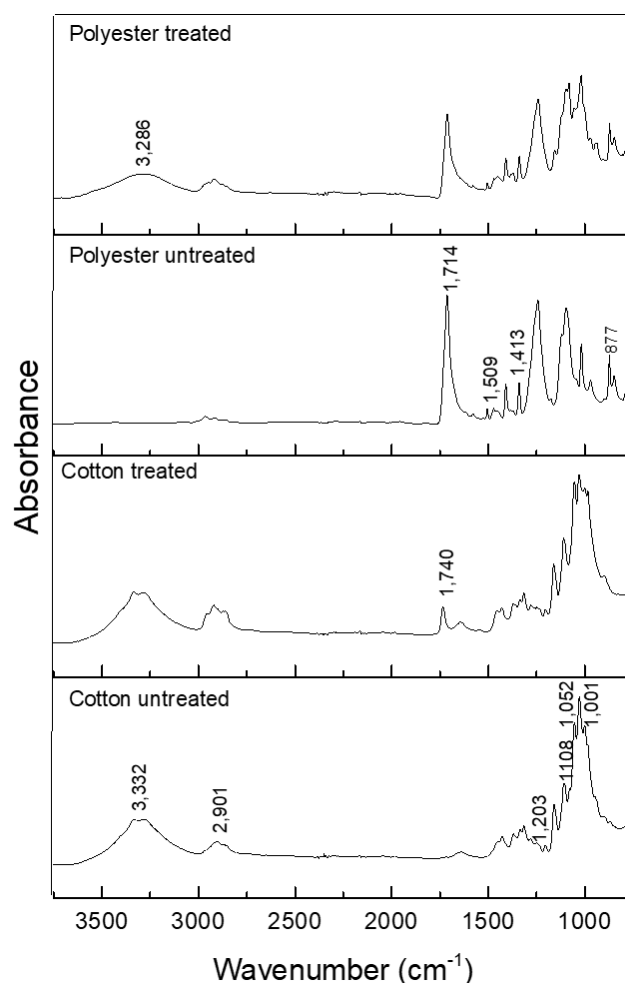
Figure 6. ATR-FTIR spectra of treated and untreated cotton and polyester textile.
