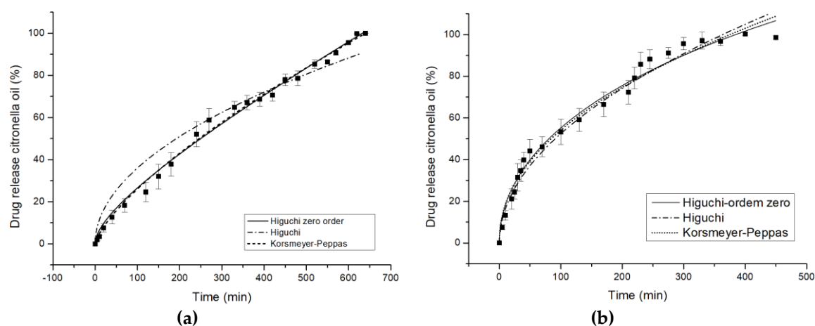
Figure 7. In vitro controlled release profiles of Higuchi zero order model, Higuchi model, and Korsmeyer-Peppas model in water at 37 °C for complex citronella essential oil applied on (a) cotton and (b) polyester.
