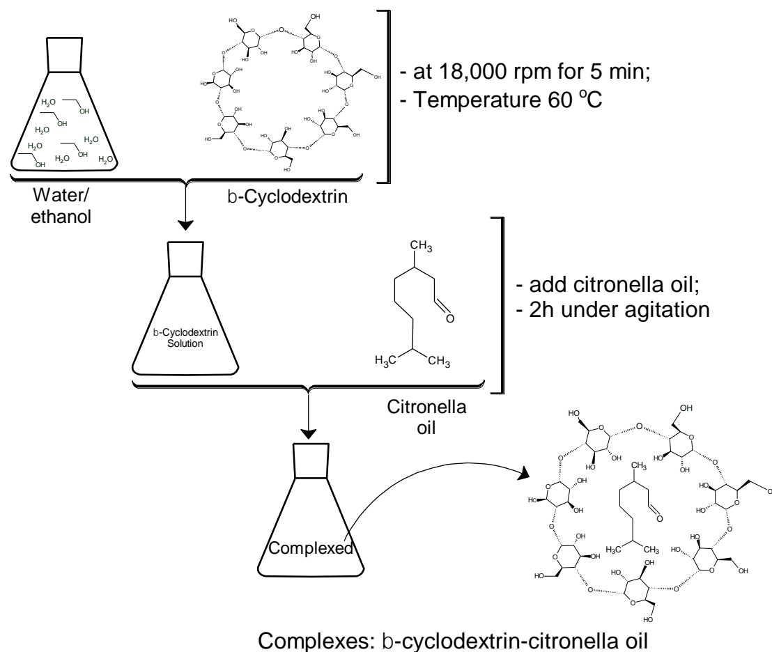
Figure 3. Experimental protocol followed for the formation of inclusion complexes CD–citronella oil.
