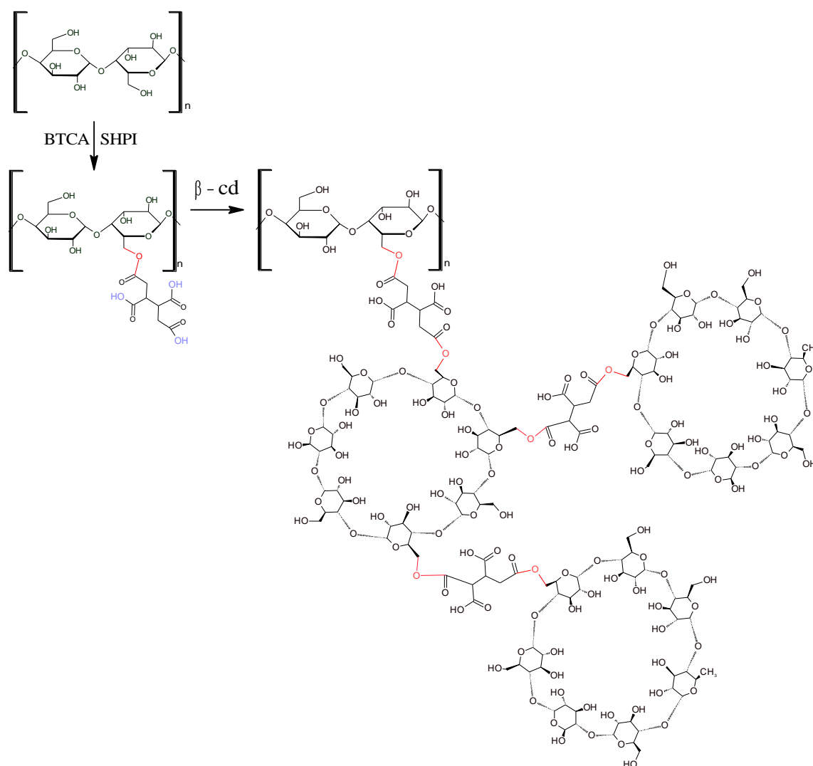
Figure 1. Grafting \beta -cyclodextrin ( \beta CD) onto hydroxyl groups of cellulose via butane-1,2,3,4-tetracarboxylic acid (BTCA) as a crosslinking agent and the catalyst sodium hypophosphite.
