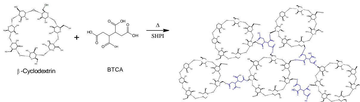
Figure 2. Complex network polymer formed between \beta CD and BTCA.
