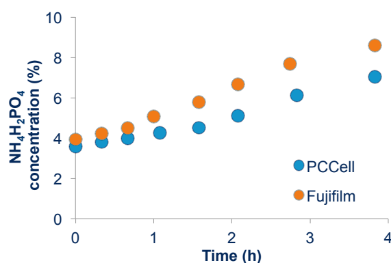
Figure 3. NH 4 H 2 PO 4 evolution in concentrated stream by ED process.
