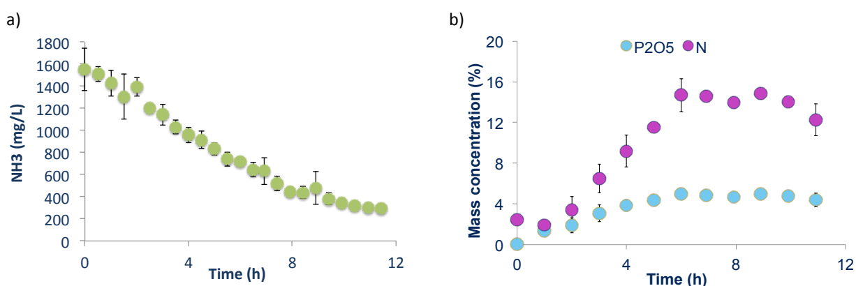
Figure 2. a) Ammonia evolution in the feed side and b) N and P 2 O 5 evolution in the stripping side over time.
