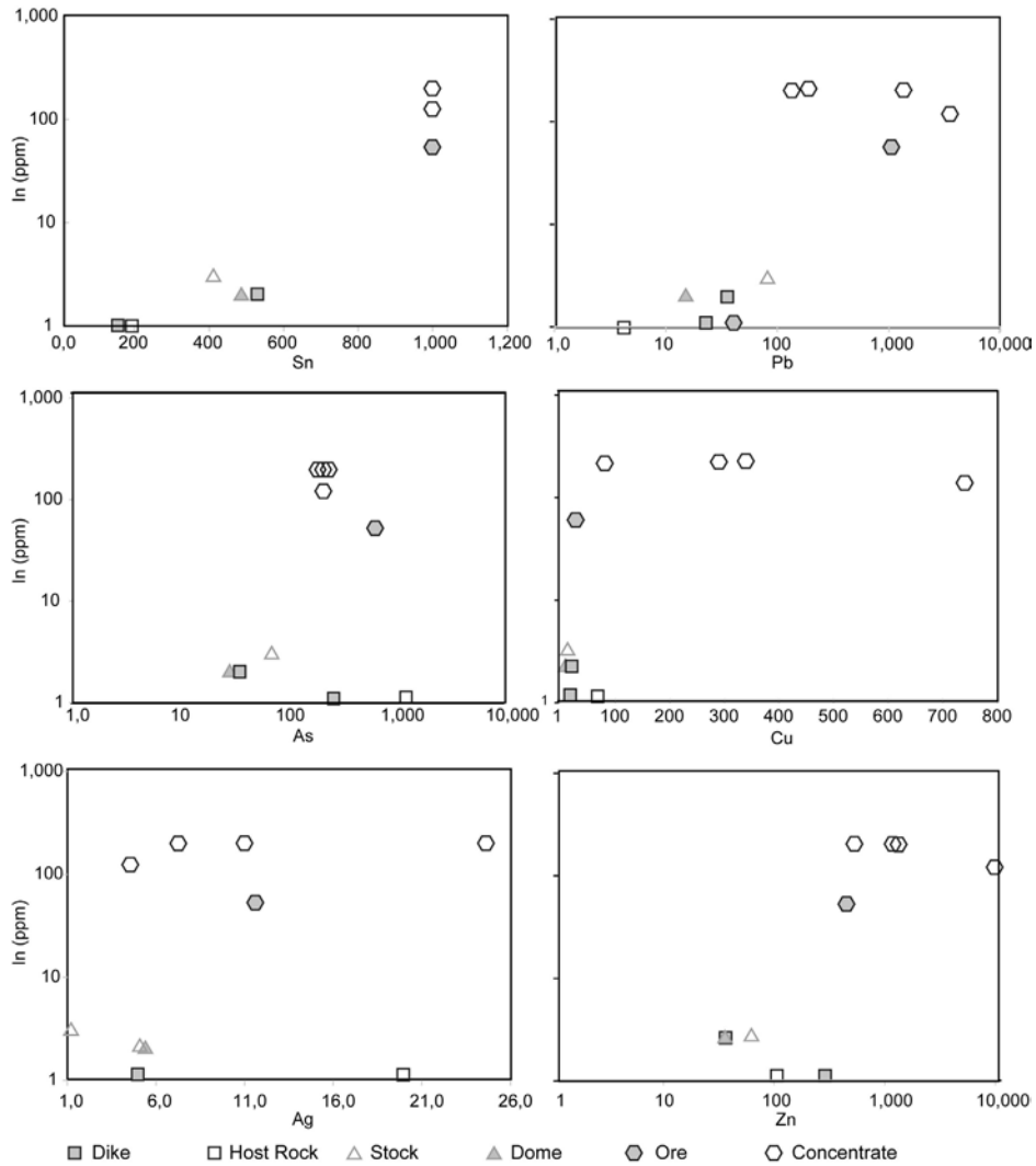
FIG. 4. Binary diagrams of Sn, Pb, As, Cu, Ag and Zn versus In in the igneous rock from the Santa Fe District, Bolivia.
