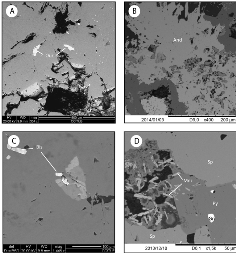
FIG. 9. Backscattered SEM images of: A. Ourayite filling cavities in a pyrite crystal; B. Acicular crystals of andorite; C. Bismuthinite crystals in a galena crystal; D. Acicular monazite crystals associated to sulfides. And: andorite; Bis: bismuthinite; Gn: galena; Our: ourayite; Py: pyrite; Sp: sphalerite; Mnz: monazite.
