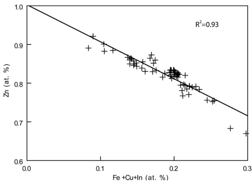
FIG. 7. Binary plots of Zn in sphalerite versus Fe+Cu+In from the Santa Fe District, Bolivia.
