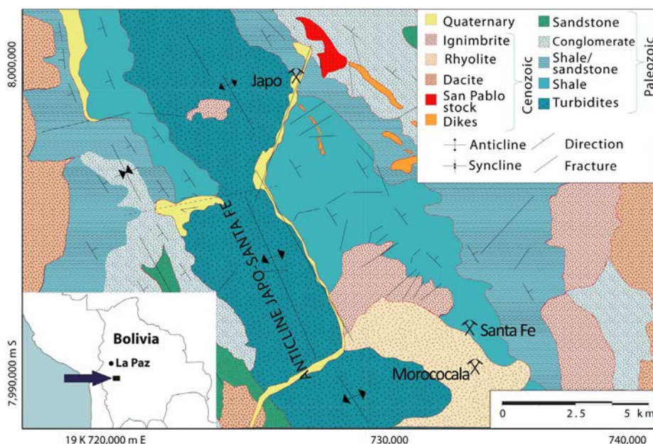
FIG. 2. Geological map of the Santa Fe District.
