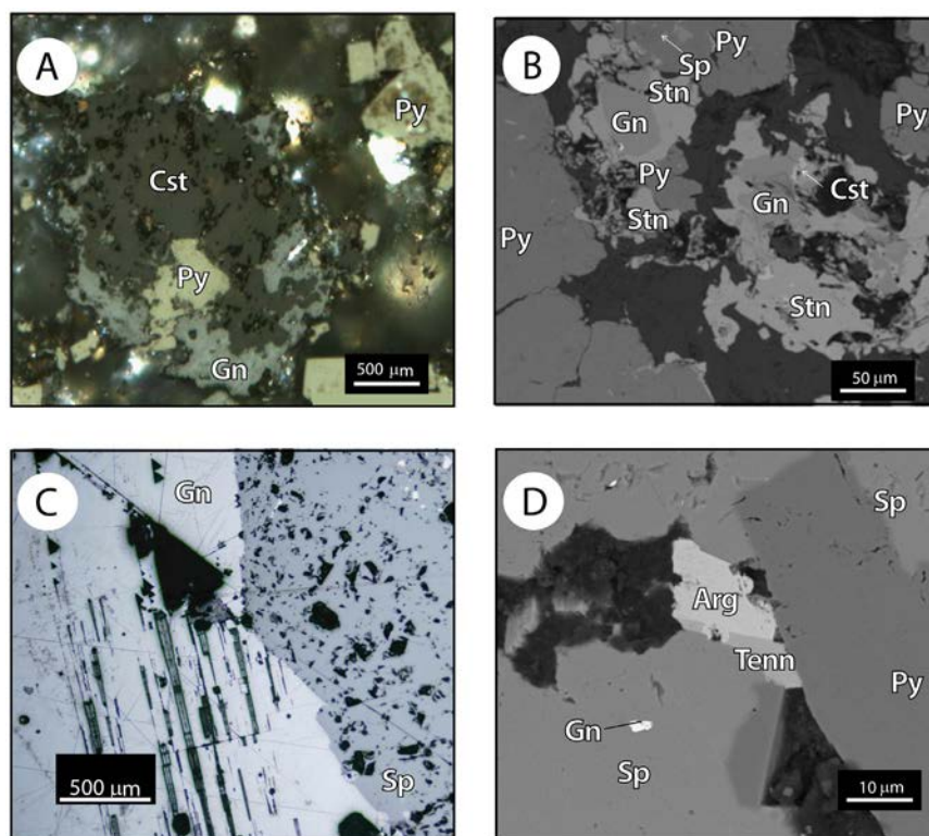
FIG. 5. A. Microphotography of the main mineral assemblage in the SFD under petrographic microscopy; B. Backscattered SEM images of the ore assemblage in the SFD; C. Microphotography of sphalerite and galena under petrographic microscopy; D. Backscattered electron SEM images of sulfosalts associated with galena, sphalerite and pyrite. Arg: argentite; Cst: cassiterite; Gn: galena; Py: pyrite; Sp: sphalerite; Stn: stannite; Tenn: tennantite.
