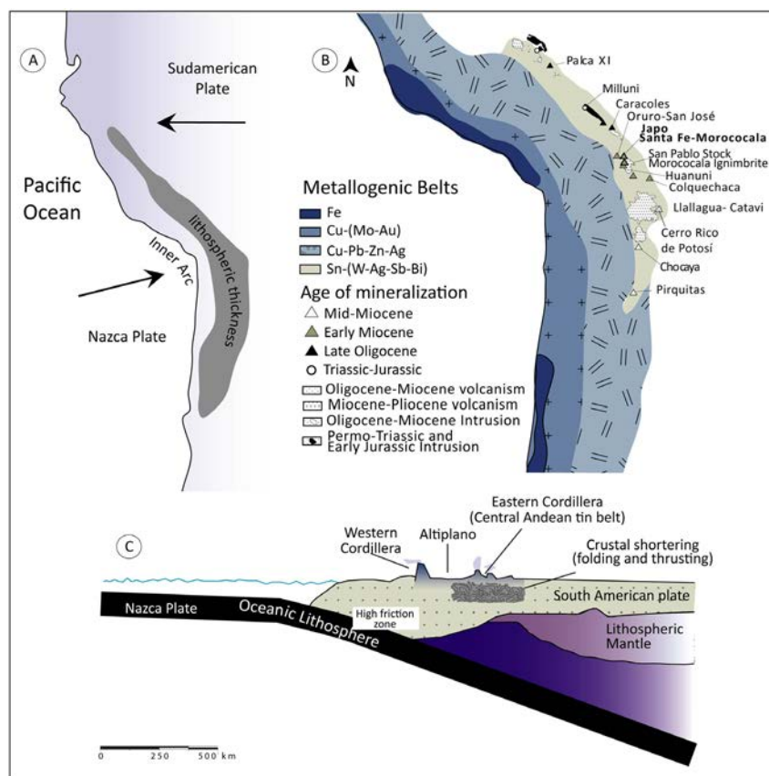
FIG. 1. Principal metallogenic belts and ore deposits of the Central Andean Tin belt (after Mlynarczyk and William-Jones, 2005). A. Plate tectonics, volcanism and lithospheric thickness; B. Relevant ore deposit with time in the Central Andean tin belt; C. Schematic cross-section of the Andean continental margin, showing the relationships.
