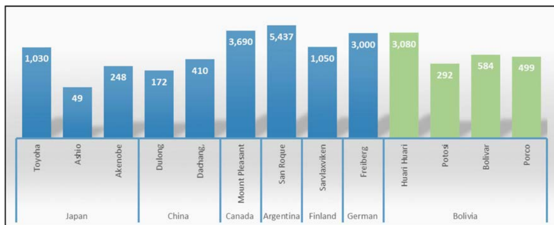
FIG. 12. Indium content of selected In-bearing deposits in ppm. Ore concentrates for Canadian, Finnish, German and Argentinian deposits, Zn concentrates for Japanese, Chinese and Bolivian deposits (Valkama et al. , 2016; Murakami and Ishihara, 2013; Dill et al. , 2013; Ishihara et al. , 2011; Cook et al. , 2011b; Sinclair et al. , 2006; Murao and Furuno, 1991; Murao et al. , 2008; Ohta, 1989; Seifert and Sandmann, 2006).
