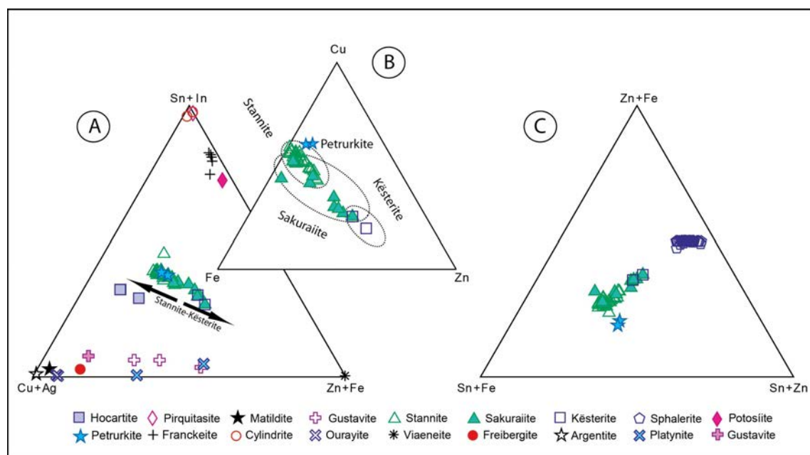
FIG. 11. A. Ternary Cu+Ag-Sn+In-Zn+Fe plot of indium-rich minerals from the SFD; B. Ternary diagram Fe-Cu-Zn, plot compositional difference between Stannite-Sakuraiite-Petrukite-K esterite-Sphalerite phases; C. Sn+Fe-Zn+Fe-Sn+Zn.
