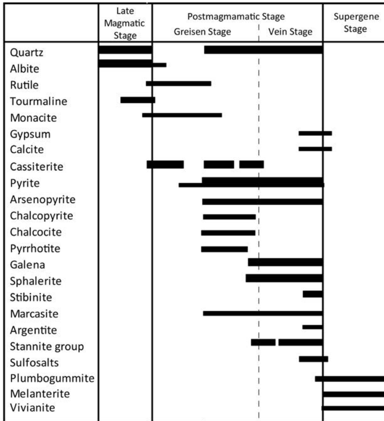
FIG. 10. Paragenetic sequence of the Santa Fe District.
