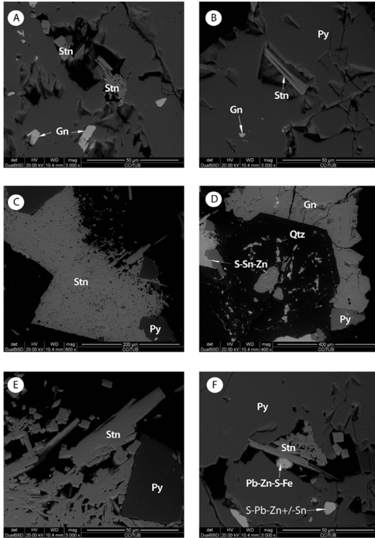
FIG. 8. Backscattered SEM images of: A. Stannite crystals filling cavities; B. Stannite crystals inside cleavage of a pyrite crystal; C. Prismatic crystals of stannite associated with pyrite; D. Ore minerals associated to euhedral quartz; E. Euhedral crystals of stannite showing tetrahedral prisms; F. minerals of stannite group with composition variable. Gn: galena; Py: pyrite; Qtz: quartz; Stn: stannite.
