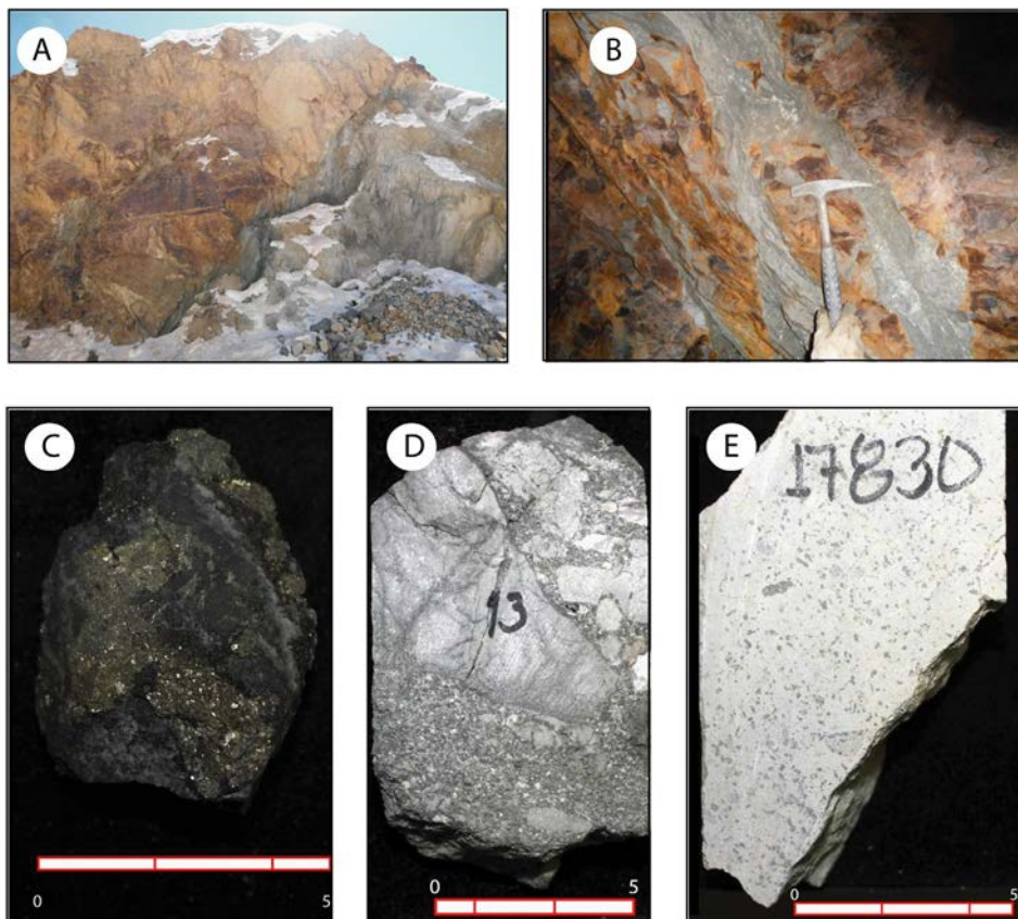
FIG. 3. Host rock and mineralization style in the Santa Fe District. A. Mineralized shear zone (gray color); B. Sulfides-bearing quartz vein in the Santa Fe mine; C. Ore minerals (Llallagua Fm.); D. Breccia with sulfides on matrix; E. Porphyry with sulfides replaced phenocrysts.
