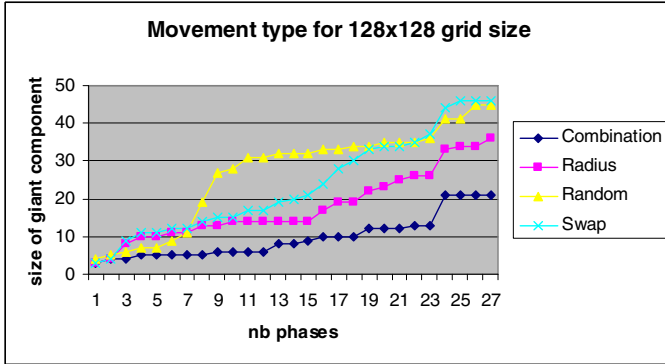
Figure 4. Performance of local movements in SA algorithm for 128x128 grid area where 64 routers were to be placed and give coverage to 192 clients.
