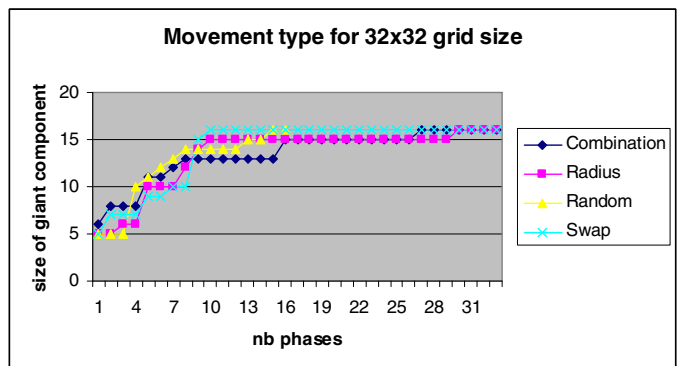
Figure 2. Performance of local movements in SA algorithm for 32x32 grid area where 16 routers were to be placed and give coverage to 48 clients.
