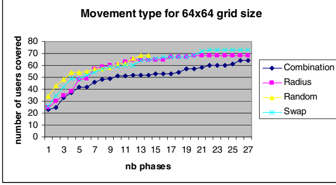
Figure 3. Performance of local movements in SA algorithm for 64x64 grid area where 32 routers were to be placed and give coverage to 96 clients.
