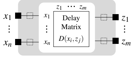
Fig. 5. Model for a combinational architecture.
