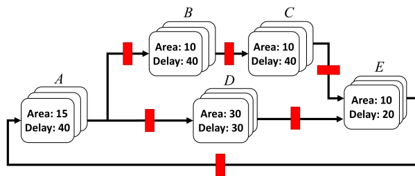
Fig. 8. Sample fork/join pipeline.
