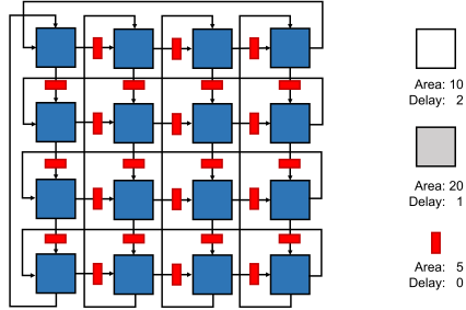
Fig. 6. Sample 4 \times 4 systolic toroidal grid.
