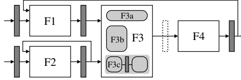
Fig. 1. Example to illustrate RTL optimizations.
