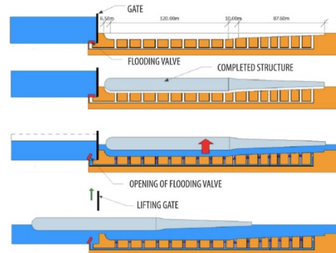
Figure 4. Fixed-mould serves both as permanent formwork and dry-dock
