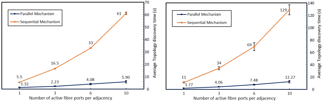
Fig. 7. Average topology discovery time comparison with Parallel / Sequential mechanisms in OTN emulated scenarios: 9-node (left) and 14-node (right).
