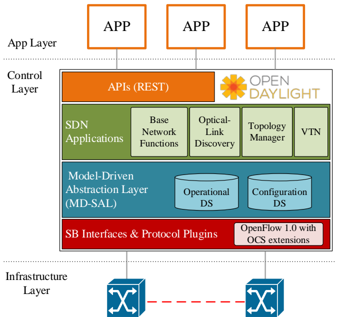
Fig. 4. SDN architecture for OTNs.
