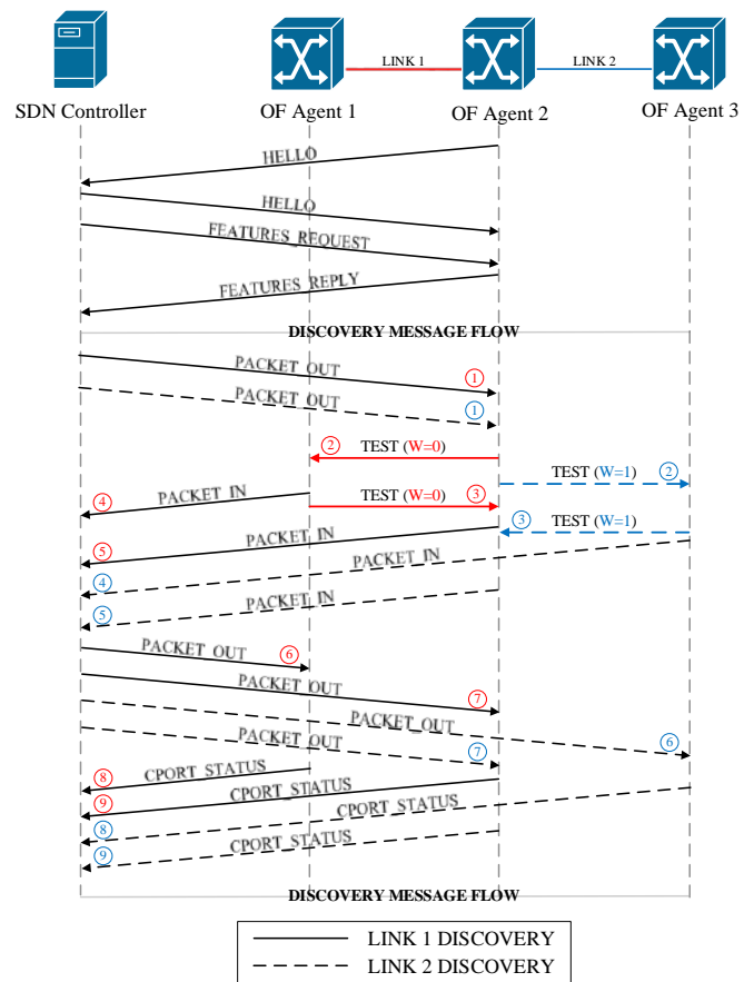
Fig. 3. Discovery Message Flow.
