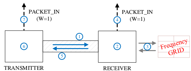
Fig. 2. Wavelength-specific Test signal mechanism.
