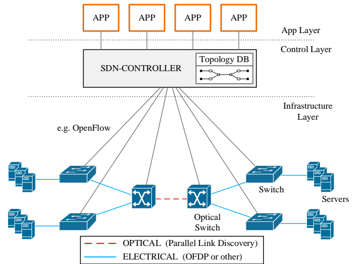
Fig. 1. SDN-enabled Hybrid Opto-Electrical Network.
