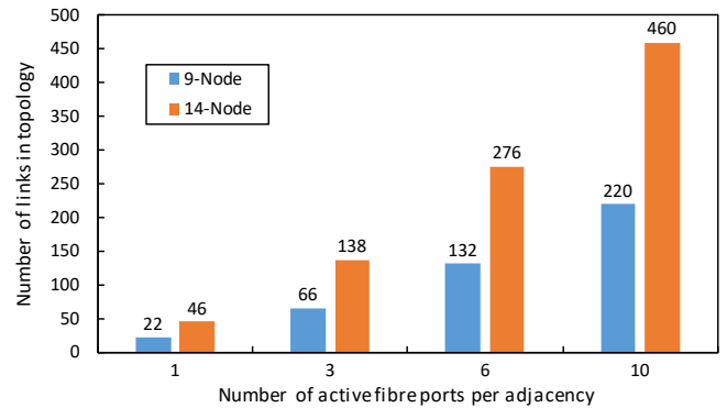
Fig. 8. Links to be discovered according to fibre ports per adjacency.
