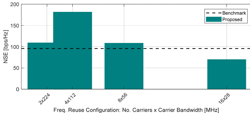
Fig. 3. NSE of the integrated backhaul network as a function of the number of carriers used to operate the network links.
