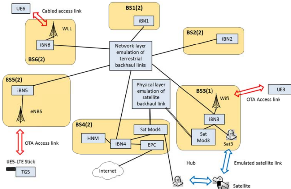
Fig. 5. Demonstration setup for evaluation of the HNM performance and its ability to improve dynamically the backhaul network capacity and resilience
