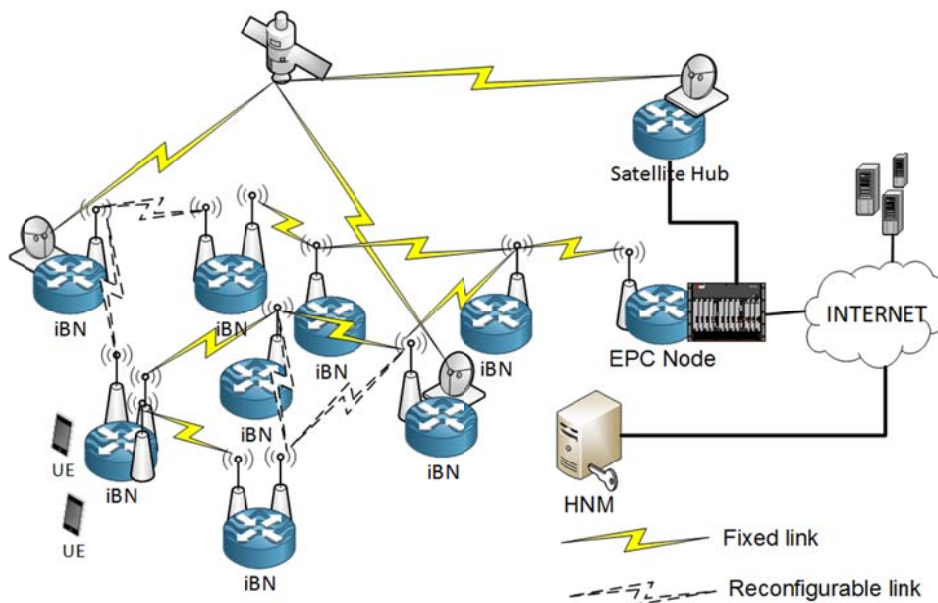
Fig. 1. SANSa System Environment
