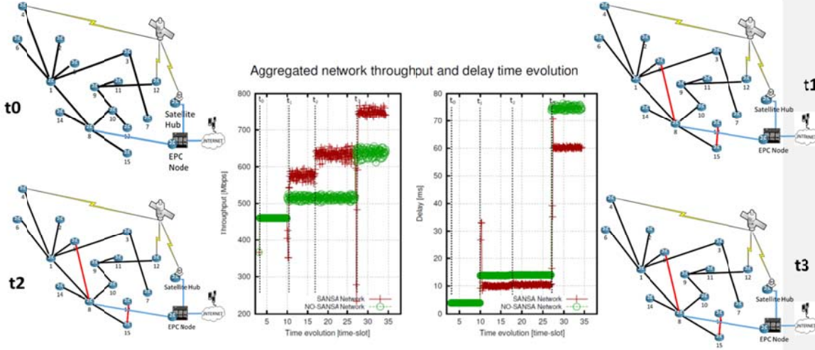
Fig. 2. Aggregated network throughput and delay over time when evaluating the reference scenario using the SANSa network with respect to a non-SANSa network.
