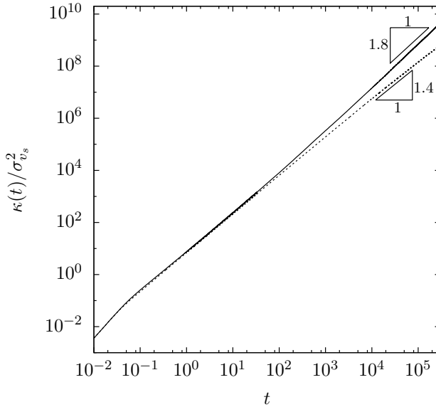
Figure 4.9: Temporal evolution of the variance in case of anomalous transport induced by both distribution and correlation for \alpha = 1.4, \beta = 1.2 (solid line) and for \alpha = 1.6, \beta = 1.9 (dashed line).
