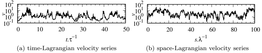
Figure 6.1: Lagrangian velocity time and space series along a particle trajectory flowing in a Darcy flow field in a \ln_K -field with \sigma_{\ln_K}^2 = 7 . The space series does not show intermittency and the time series does, the velocity series shows long time periods at low velocities and short time period at high velocities.
