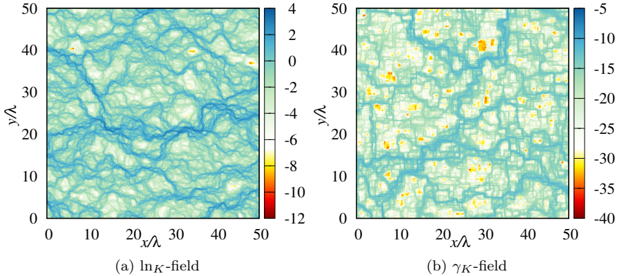
Figure 6.4: Individual realization of the log of the velocity magnitude for flow in heterogeneous media for a \ln_K -field ( \sigma_{\ln K}^2 = 7 ) and for a \gamma_K -field ( \alpha = 0.1 ). Note the great proportion of low velocities in the \gamma_K -field.
