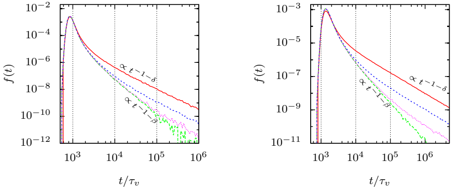
Figure 3.6: First passage time distributions at x_c = 5 \times 10^2 \ell_c for (left panel) \beta = 3/2 , \delta = 1/2 , and (right panel) \beta = 5/4 and \delta = 1/4 for (red solid line) \gamma = 10^{-3} \tau_v^{-1} , (blue short dashed) \gamma = 10^{-4} \tau_v^{-1} , (pink dotted) \gamma = 10^{-5} \tau_v^{-1} and (green long-dashed) \gamma = 0 . The advection time scale is \tau_v = 10^{-1} . The black vertical dashed lines mark (left to right) \tau_\gamma = 10^3 \tau_v , 10^4 \tau_v and 10^5 \tau_v .
