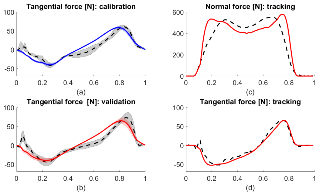
Figure 1: Left: Calibration results (a) and validation results (b) of the tangential contact model for Subject 1: mean and standard deviation of experimental data (dashed black), calibration results (blue), and validation results (red). Right: Results of normal (c) and tangential (d) ground reaction forces obtained when tracking walking motion for Subject 3, using the calibrated contact model parameter values: experimental force measurements (dashed black) and predicted force values (red). Results are shown for normalized stance time.
