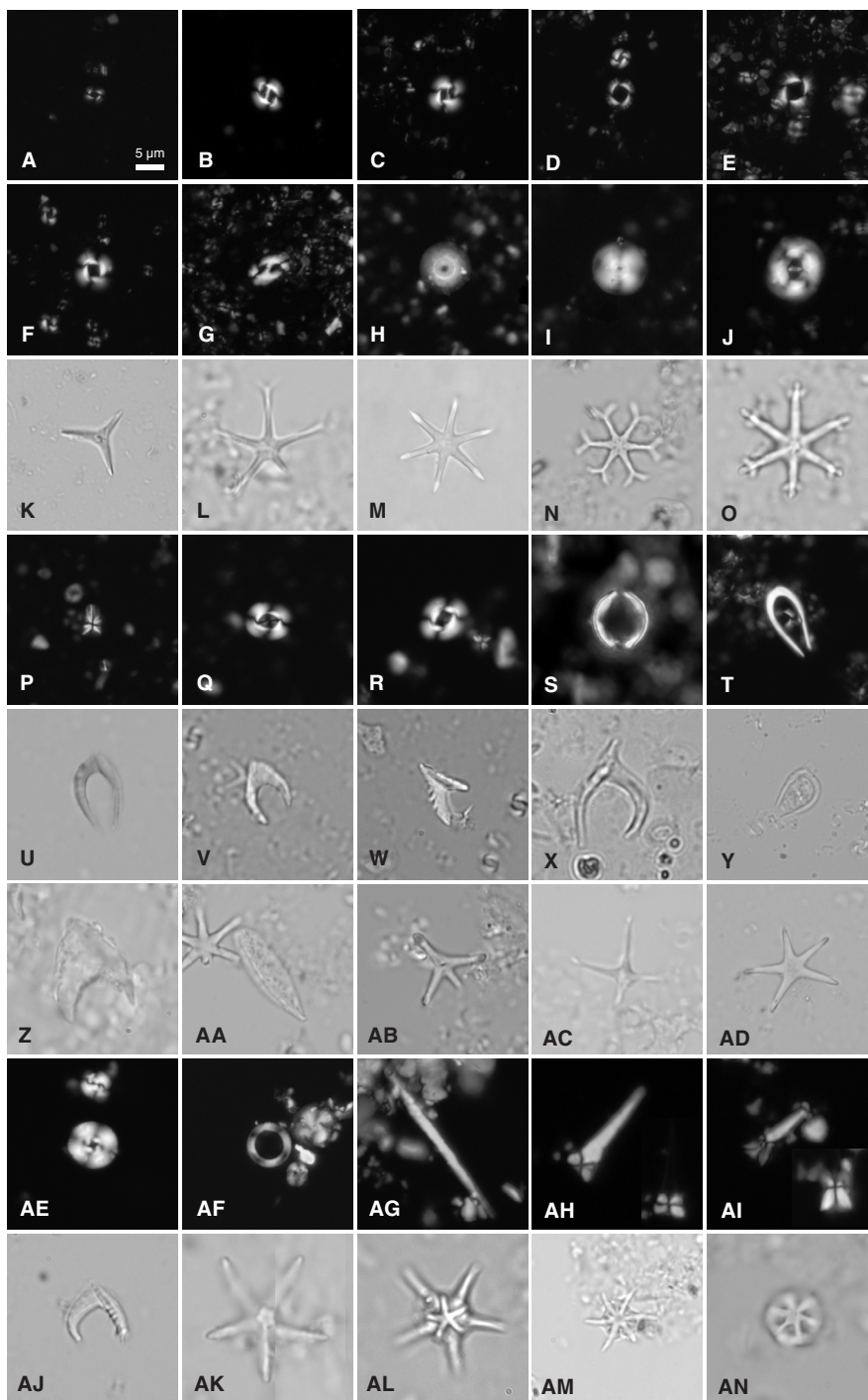
Figure F31. Calcareous nannofossils from selected Expedition 363 sites. A. Emiliania huxleyi ; U1485A-1H-CC. B. Gephyrocapsa oceanica ; U1485A-1H-CC. C. Gephyrocapsa >5.5 \mu m; U1486B-8H-CC. D,E. Pseudoemiliania lacunosus ; (D) U1489C-2H-6, 60 cm, (E) U1489B-2H-6, 75 cm. F. Reticulofenestra asanoi ; U1483A-9H-6, 50 cm. G. Helicosphaera sellii ; U1486B-10H-CC. H, I. Calcidiscus macintyreii ; (H) U1486B-12H-CC, (I) U1486B-19H-CC. J. Coccolithus pelagicus ; U1486B-15H-CC. K. Discoaster triradiatus ; U1482A-18H-CC. L. Discoaster pentaradiatus ; U1489C-8H-4, 60 cm. M. Discoaster brouweri ; U1482A-12H-2, 75 cm. N. Discoaster variabilis ; U1489B-12H-CC. O. Discoaster surculus ; U1482B-38H-CC. P. Sphenolithus abies ; U1483A 31H-CC. Q, R. Reticulofenestra pseudoumbilicus ; (Q) U1483A-31H-CC, (R) U1489B-10H-CC. S. Scyphosphaera globulata ; U1488A-14H-2, 60 cm. T, U. Ceratolithus cristatus ; (T) U1489B-3H-CC, (U) U1428B-18H-CC. V, W. Ceratolithus armatus ; (V) U1482B-27H-4, 50 cm, (W) U1482B-27H-CC. X. Amaurolithus tricorniculatus ; U1482A-22H-6, 75 cm. Y. Amaurolithus delicatus ; U1482B-27H-CC. Z. Amaurolithus primus ; U1489C-22H-CC. AA. Triquetrorhabdulus carinatus ; U1489C-31F-CC. AB. Discoaster sp.; U1486B-22H-6, 81 cm. AC. Discoaster tamalis ; U1489B-6H-CC. AD. Discoaster asymmetricus ; U1483A-31H-CC. AE. Cyclicargolithus floridanus ; U1489C-38X-6, 40 cm. AF. Coronocyclus nitescens ; U1489C-42X-4, 30 cm. AG. Triquetrorhabdulus carinatus ; U1489C-41X-CC. AH. Sphenolithus heteromorphus ; U1489C-41X-CC. AI. Sphenolithus belemnus ; U1489C-41X-CC. AJ. Nicklithus amplificus ; U1482B-33H-CC. AK. Discoaster quinquerramus ; U1489C-24H-CC. AL. Discoaster berggrenii ; 1482C-41X-CC. AM. Catinaster calyculus ; U1489C-31F-CC. AN. Catinaster coalitus ; U1489C-30F-CC.
