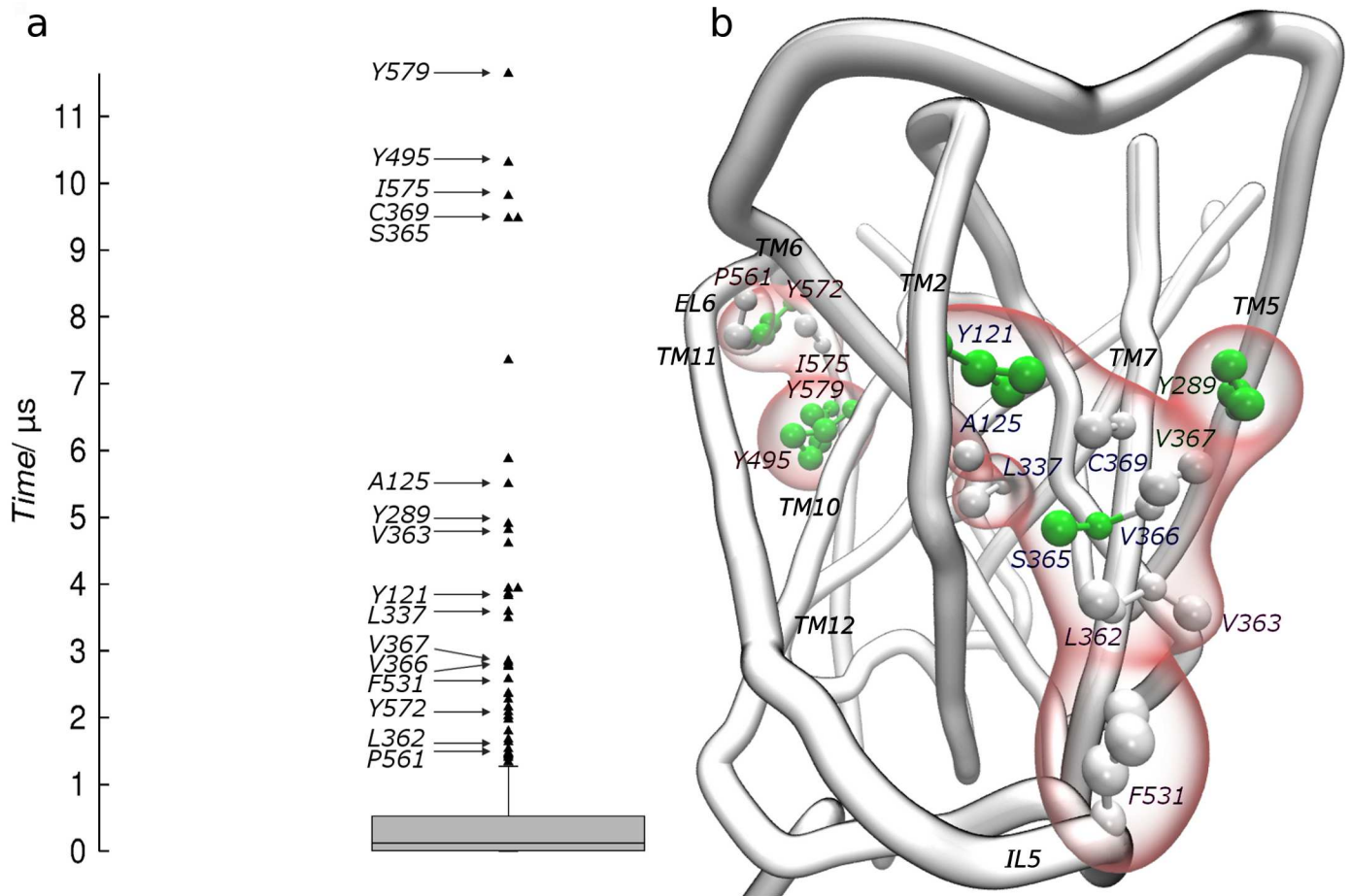
Fig 2. Outliers characterization. (a) Distribution of t_{max} obtained merging eleven data-sets from SYS1-3 in a unique population. The box-plot diagram shows the outliers located above 1.3 μs (black triangles). (b) Corresponding amino acids are only labeled for the sixteen outliers matching a reproducible cholesterol density, and are mapped on the three-dimensional representation of the SERT surface. Outliers are colored by residue type and contoured by a red surface. Labels follow the site-based coloring scheme shown in Fig 3.
