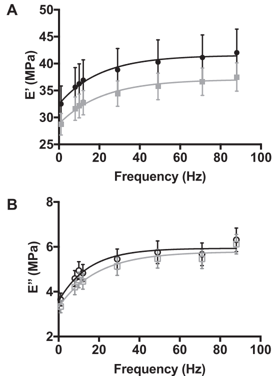
Fig. 2. A) Storage modulus ( E' ) of healthy ( \bullet ) and OA ( \blacksquare ) cartilage with 95% confidence intervals, B) Loss modulus ( E'' ) of healthy ( \circ ) and OA ( \square ) cartilage with 95% confidence intervals; H n = 22, OA n = 37.
