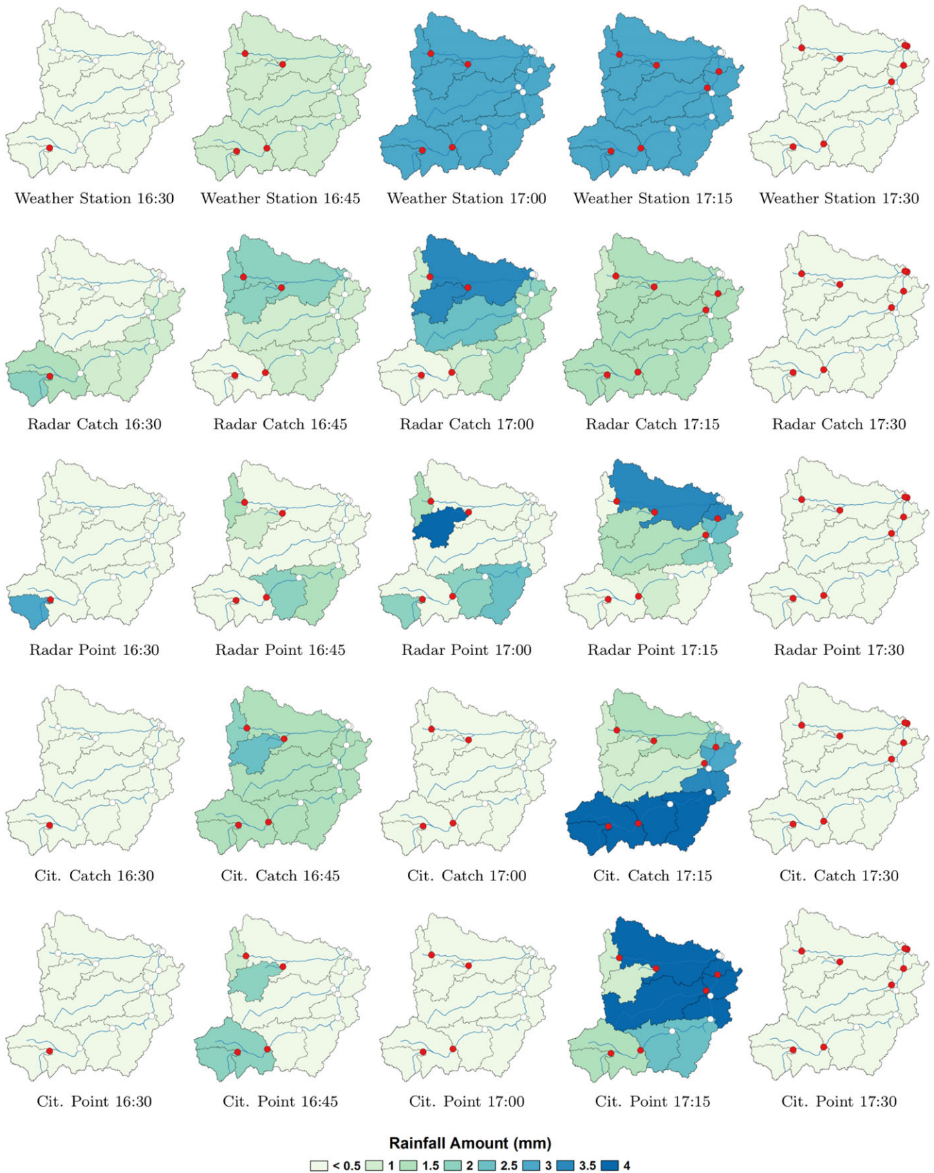
FIGURE 6 Temporal development of the event on September 13, 2016, event for the different precipitation methods: White circles show no water temperature surge; red indicate >1° rise in water temperature for that site. Colours indicate precipitation in mm. Maps created in GIS by colouring in each logger nested catchment with corresponding precipitation amount for time period
