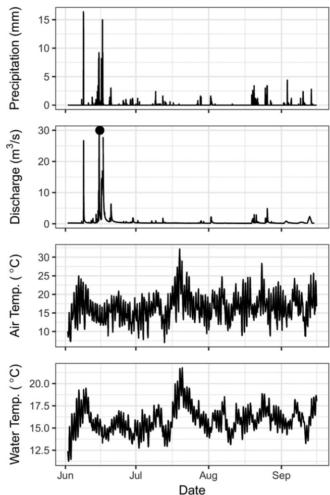
FIGURE 2 Time series for site R1 (see Figure 1) showing water temperature, air temperature, and precipitation as recorded at the weather station, and discharge as recorded at the catchment outlet. The black dot on the discharge graph shows a particularly large event that peaked at 62 m 3 /s, outside the limits of the y-axis
