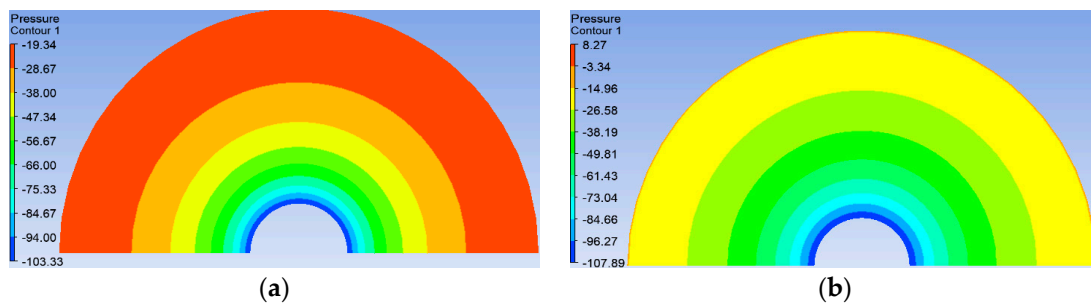
Figure 7. The contour slice of pressure of incompressible and compressible flow, t = 1.0 s, R = 50 m. (a) Incompressible flow; (b) compressible flow.
