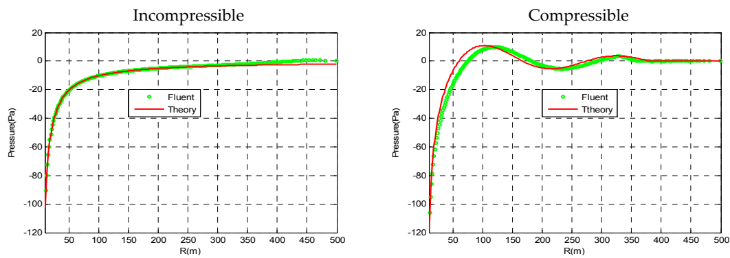
Figure 6. The relationship between pressure vs. radii in incompressible and compressible flow when t = 1.0 s.
