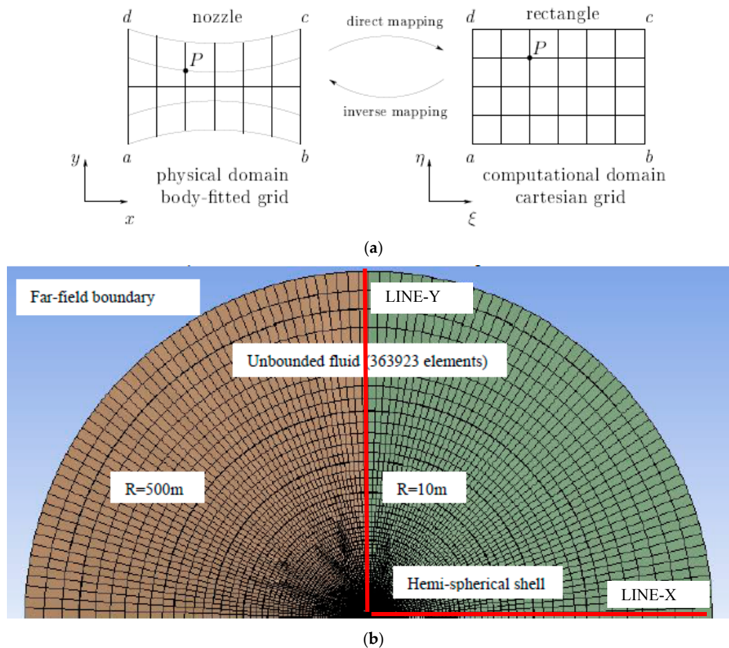
Figure 3. Spherical symmetry model of a hemispherical shell vibrating in unbounded fluid. (a) Transformation of random domain to computational domain; (b) mesh and boundary conditions.
