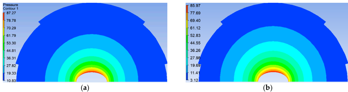
Figure 17. The contour slice of pressure of incompressible and compressible flow, t = 0.65 s, R = 50 m. (a) Incompressible flow; (b) compressible flow.
