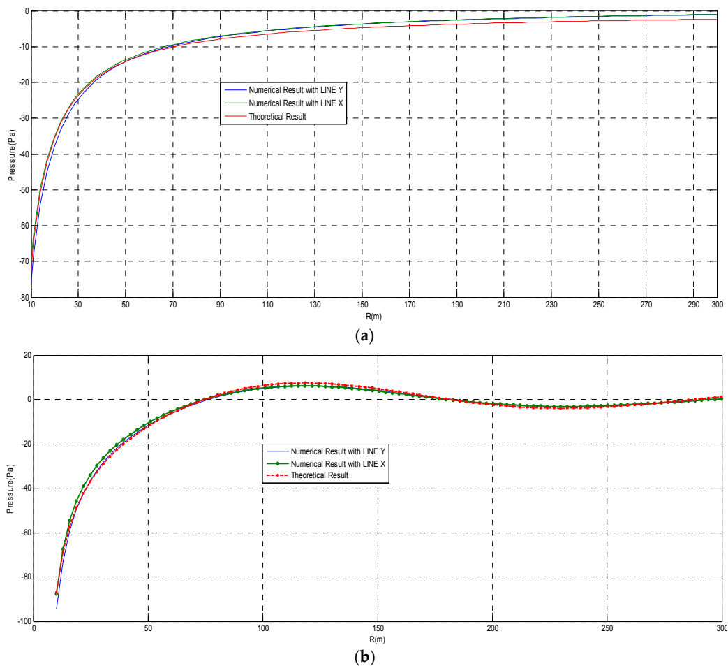
Figure 11. The relationship between pressure vs. time of incompressible and compressible flow. (a) Incompressible flow; (b) compressible flow.
