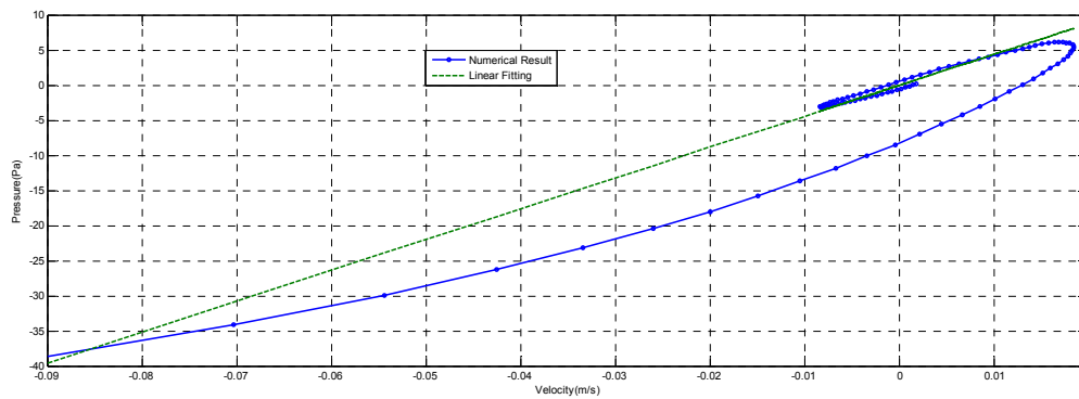
Figure 13. Velocity vs-pressure graph in compressible flow, with ellipse A = 10 , B = 8 .
