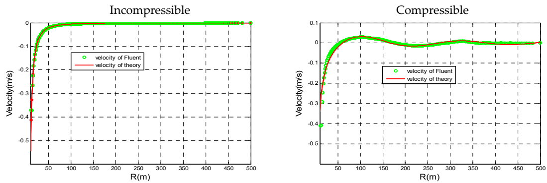
Figure 4. The relationship between velocity vs. radius of incompressible and compressible fluid when t = 1.0 s.
