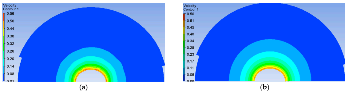
Figure 10. The contour slice of velocity of incompressible and compressible flow, t = 1.0 s, R = 50 m. (a) Incompressible flow; (b) compressible flow.
