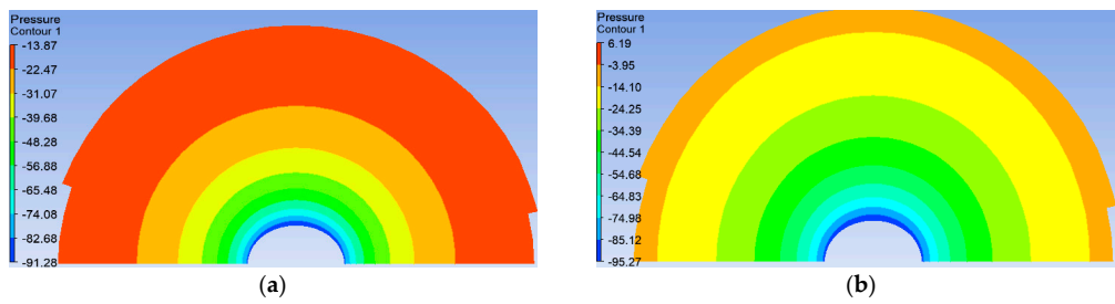
Figure 12. The contour slice of pressure of incompressible and compressible flow, t = 1.0 s, R = 50 m. (a) Incompressible flow; (b) compressible flow.
