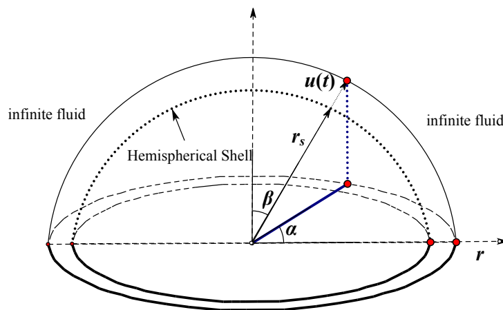
Figure 2. The state of the vibration of a hemispherical shell.
