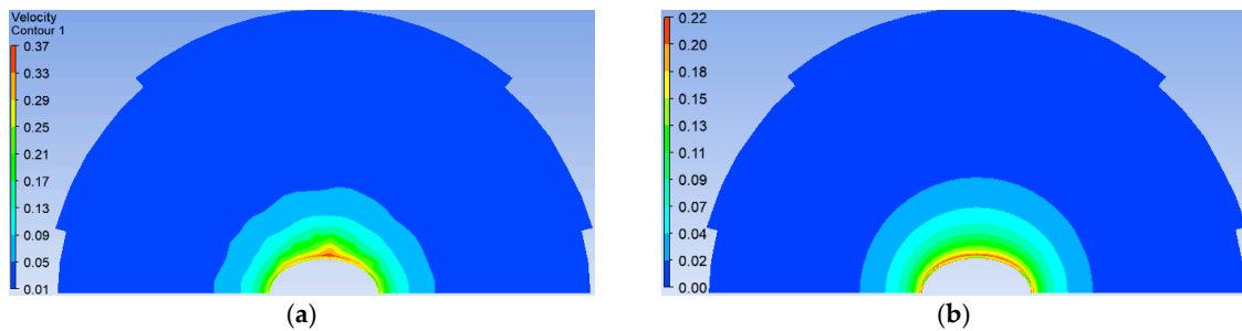
Figure 15. The contour slice of velocity of incompressible and compressible flow, t = 0.65 s, R = 50 m. (a) Incompressible flow; (b) compressible flow.
