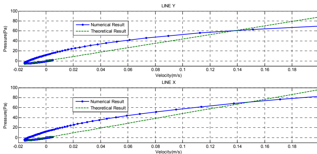
Figure 18. The relationship between velocity vs. pressure in compressible flow, with ellipses A = 10 , B = 8 .
