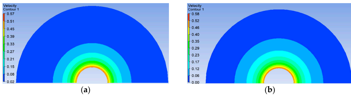
Figure 5. The contour slice of velocity of incompressible and compressible flow, t = 1.0 s, R = 50 m. (a) Incompressible flow; (b) compressible flow.
