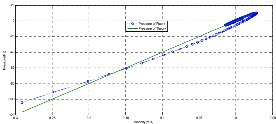
Figure 8. The relationship between pressure vs. velocity in compressible flow, when t = 1.0 s.
