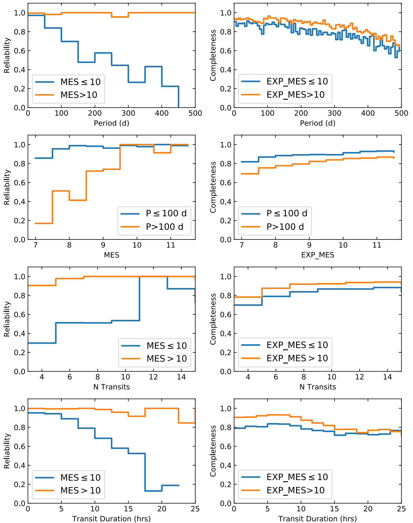
Figure 9. Reliability (left) and completeness (right) of the DR25 catalog plotted as a function of period, MES, number of transits, and transit duration. In each case the blue line is for those with MES \leq 10 or period \leq 100 days. The orange line shows the completeness or reliability for the rest of the population (see the legend for each panel). EXP\_MES is the expected MES (see Christiansen 2017; see also Section 7.3.1).
