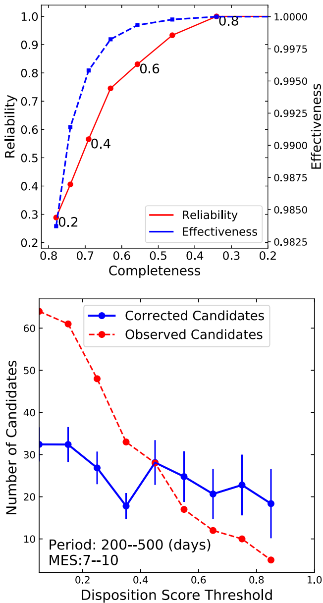
Figure 13. Top: reliability (red) and effectiveness (blue) of the DR25 catalog as a function of completeness for MES \leq 10 and periods between 200 and 500 days for the PCs that result when using different disposition score thresholds (shown as black numbers) to select the PCs. Higher disposition score thresholds result in higher reliability but lower completeness. Note that the completeness axis increases to the left. Bottom: number of PCs (in red) in the same period and MES space when making a cut on different disposition scores. The blue line corrects the number of candidates for the completeness and reliability. The error bars only reflect a Poisson error based on the number of observed planet candidates shown in red.
