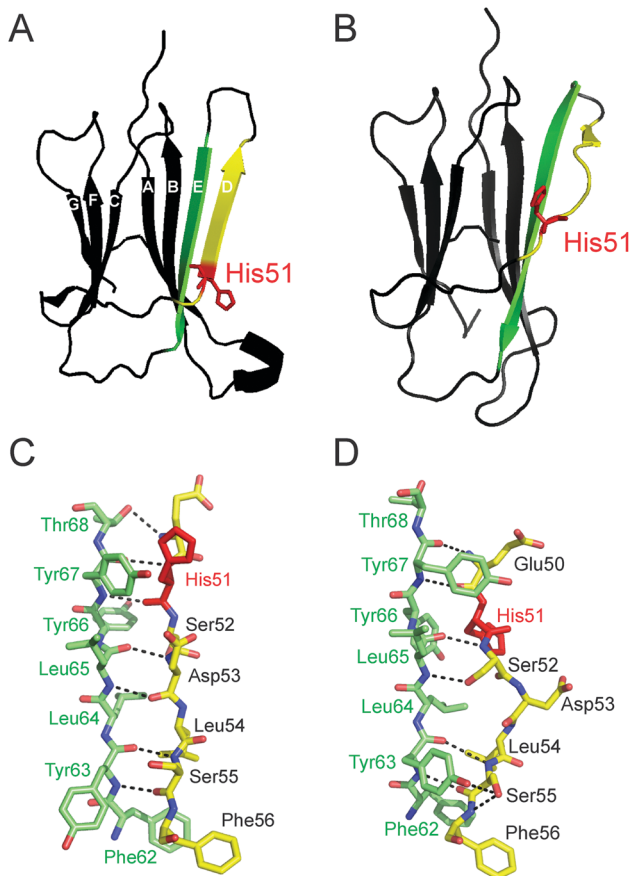
Fig. 1 Ribbon structures of wild-type human \beta_2m highlighting the different conformations of the D strand (yellow) between (A) monomeric, apo- \beta_2m (PDB file: 1LDS) 7 and (B) the MHC 1-bound holo form (PDB file: 2X70). The hydrogen bond contacts (black dashed lines) between the D- (yellow) and E- (green) strands of \beta_2m are shown in the case of both monomeric, apo- \beta_2m (C) and the MHC 1-bound holo form (D). The location of His51 (red) is highlighted on each structure.
