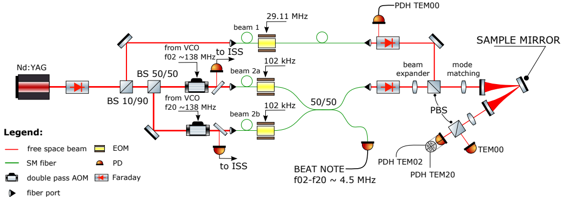
FIG. 3. The experimental setup for the multi-mode measurement involves a Nd:YAG laser (far left) and an in-vacuum high-finesse cavity (far right). In order to avoid multiple lasers, and the multiple sources of frequency and intensity noise they would introduce, a single laser beam is split into 3 paths, 2 of which are shifted in frequency (with AOMs), and each of which is independently phase modulated at its own radio frequency (with EOMs). The laser frequency is controlled to lock the TEM00 mode to the cavity length while the TEM02 and TEM20 modes are locked to the cavity by controlling their frequency differences with respect to the laser frequency. The primary output of the experiment is the difference between the TEM02 and TEM20 resonant frequencies (labeled BEAT NOTE), changes in which are dominated by the coating thermal noise of the sample.
